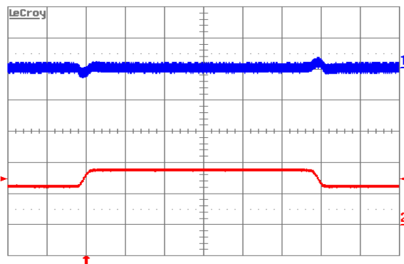
Figure 8. Output voltage response to load current step-change (12.5A–18.75A–12.5A) at V_{\text{in}}=48\text{V} . Top trace: output voltage (100mV/div.). Bottom trace: load current (10A/div.). Current slew rate: 0.1A/ \mu\text{s} . C_o=1\mu\text{F cer}+10\mu\text{F tant} . Time scale: 0.2ms/div.
