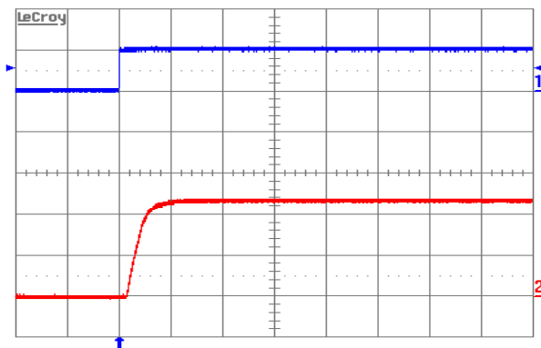
Figure 7. Turn-on transient at full rated load current (resistive) plus 30,000 \mu\text{F} at V_{\text{in}} = 48\text{ V} , triggered via ON/OFF pin. Top trace: ON/OFF signal (5 V/div.). Bottom trace: Output voltage (0.5 V/div.). Time scale: 5 ms/div.
