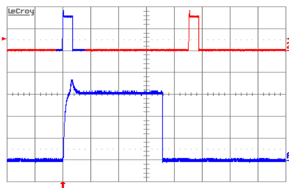
Figure 15. Load current (top trace, 20 A/div., 50 ms/div.) into a 10\ \text{m}\Omega short circuit during restart, at V_{in} = 48\text{V} . Bottom trace (10 A/div., 5 ms/div.) is an expansion of the on-time portion of the top trace
