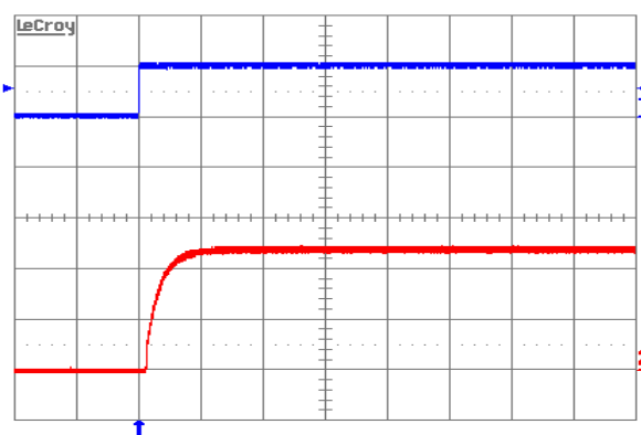
Figure 6. Turn-on transient at full rated load current (resistive) with C_o=1\mu\text{F} cer+ 10\mu\text{F} tant at V_{in} = 48\text{ V} , triggered via ON/OFF pin. Top trace: ON/OFF signal (5 V/div.). Bottom trace: Output voltage (0.5 V/div.). Time scale: 5 ms/div.
