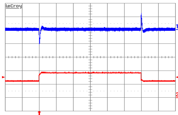
Figure 9. Output voltage response to load current step-change (12.5A–18.75A–12.5A) at V_{\text{in}}=48\text{V} . Top trace: output voltage (100 mV/div.). Bottom trace: load current (10A/div.). Current slew rate: 5A/ \mu\text{s} . C_o=470\mu\text{F POS}+1\mu\text{F cer} . Time scale: 0.2ms/div.
