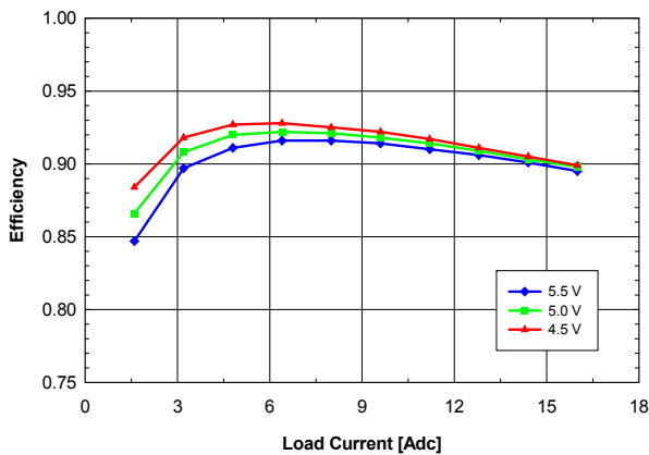
Fig. 1.8V.2: Efficiency vs. load current and input voltage for V_{out} = 1.8 V converter mounted vertically with air flowing from pin 10 to pin 1 at a rate of 200 LFM (1 m/s) and T_a = 25 °C.
