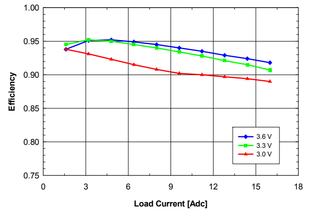
Fig. 2.5V.3: Efficiency vs. load current and input voltage for V_{out} = 2.5 V converter mounted vertically with air flowing from pin 10 to pin 1 at a rate of 200 LFM (1 m/s) and T_a = 25 °C.
