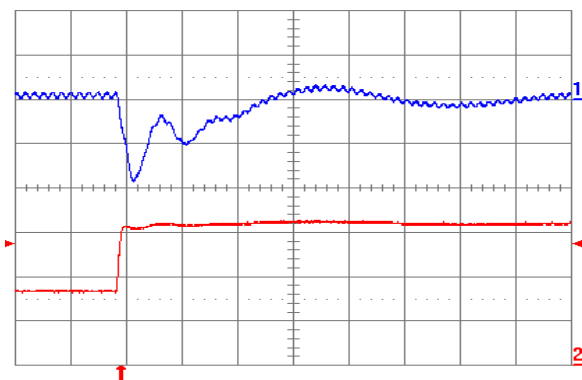
Fig. 3.3V.6: Output voltage response for V_{out} = 3.3 V to positive load current step change from 8 A to 16 A with slew rate of 5 A/ \mu s at V_{in} = 5 V. Top trace: output voltage (100 mV/div.); Bottom trace: load current (5 A/div.). C_o = 100 \mu F ceramic + 1 \mu F ceramic. Time scale: 20 \mu s/div.
