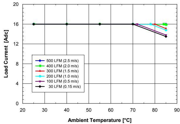
Fig. 2.5V.1: Available load current vs. ambient temperature and airflow rates for V_{out} = 2.5 V converter mounted vertically with V_{in} = 5 V, air flowing from pin 10 to pin 1, and maximum MOSFET temperature \leq 120 °C.
