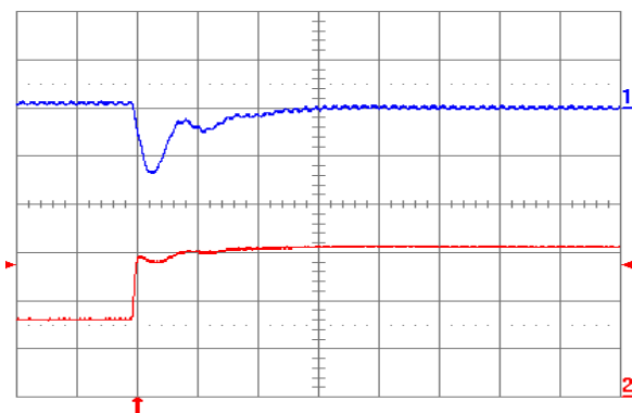
Fig. 1.2V.6: Output voltage response for V_{out} = 1.2 V to positive load current step change from 8 A to 16 A with slew rate of 5 A/ \mu s at V_{in} = 5 V. Top trace: output voltage (100 mV/div.); Bottom trace: load current (5 A/div.). C_o = 100 \mu F ceramic + 1 \mu F ceramic. Time scale: 20 \mu s/div.
