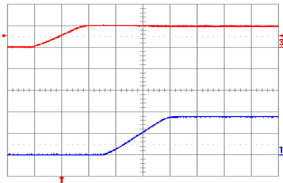
Fig. 1.8V.4: Turn-on transient for V_{out} = 1.8 V with application of V_{in} at full rated load current (resistive) and 100 \mu F external capacitance at V_{in} = 5 V. Top trace: V_{in} (5 V/div.); Bottom trace: output voltage (1 V/div.); Time scale: 2 ms/div.
