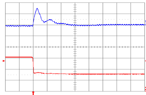
Fig. 1.5V.7: Output voltage response for V_{out} = 1.5 V to negative load current step change from 16 A to 8 A with slew rate of -5 A/ \mu s at V_{in} = 5 V. Top trace: output voltage (100 mV/div.); Bottom trace: load current (5 A/div.). C_o = 100 \mu F ceramic + 1 \mu F ceramic. Time scale: 20 \mu s/div.
