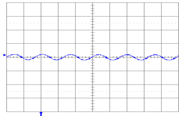
Fig. 1.8V.5: Output voltage ripple (20 mV/div.) at full rated load current into a resistive load with external capacitance 100 \mu F ceramic + 1 \mu F ceramic and V_{in} = 5 V for V_{out} = 1.8 V. Time scale: 2 \mu s/div.
