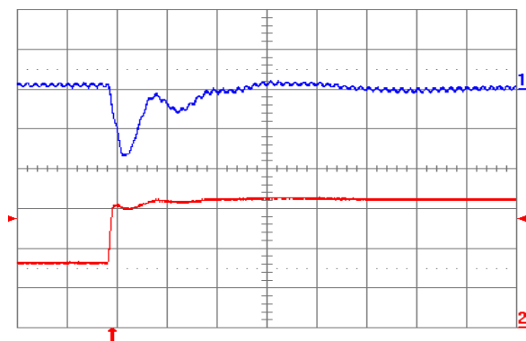
Fig. 2.0V.6: Output voltage response for V_{out} = 2.0 V to positive load current step change from 8 A to 16 A with slew rate of 5\text{ A}/\mu\text{s} at V_{in} = 5 V. Top trace: output voltage (100 mV/div.); Bottom trace: load current (5 A/div.). C_o = 100\text{ }\mu\text{F} ceramic + 1\text{ }\mu\text{F} ceramic. Time scale: 20 \mu\text{s} /div.
