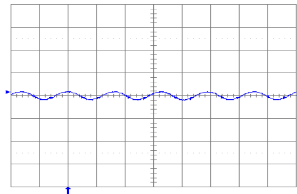
Fig. 1.5V.5: Output voltage ripple (20 mV/div.) at full rated load current into a resistive load with external capacitance 100 \mu F ceramic + 1 \mu F ceramic and V_{in} = 5 V for V_{out} = 1.5 V. Time scale: 2 \mu s/div.
