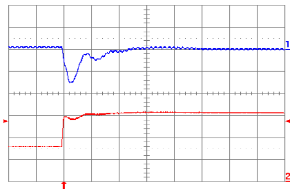
Fig. 1.5V.6: Output voltage response for V_{out} = 1.5 V to positive load current step change from 8 A to 16 A with slew rate of 5 A/ \mu s at V_{in} = 5 V. Top trace: output voltage (100 mV/div.); Bottom trace: load current (5 A/div.). C_o = 100 \mu F ceramic + 1 \mu F ceramic. Time scale: 20 \mu s/div.
