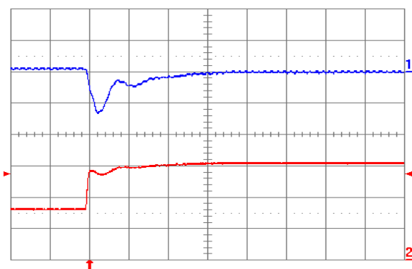
Fig. 1.0V.6: Output voltage response for V_{out} = 1.0 V to positive load current step change from 8 A to 16 A with slew rate of 5 A/ \mu s at V_{in} = 5 V. Top trace: output voltage (100 mV/div.); Bottom trace: load current (5 A/div.). C_o = 100 \mu F ceramic + 1 \mu F ceramic. Time scale: 20 \mu s/div.
