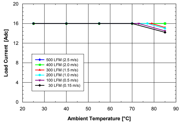
Fig. 1.5V.1: Available load current vs. ambient temperature and airflow rates for V_{out} = 1.5 V converter mounted vertically with V_{in} = 5 V, air flowing from pin 10 to pin 1, and maximum MOSFET temperature \leq 120 °C.
