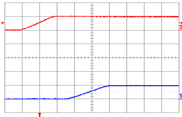
Fig. 1.0V.4: Turn-on transient for V_{out} = 1.0 V with application of V_{in} at full rated load current (resistive) and 100 \mu F external capacitance at V_{in} = 5 V. Top trace: V_{in} (5 V/div.); Bottom trace: output voltage (0.5 V/div.); Time scale: 2 ms/div.
