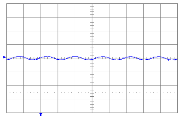
Fig. 1.0V.5: Output voltage ripple (20 mV/div.) at full rated load current into a resistive load with external capacitance 100 \mu F ceramic + 1 \mu F ceramic and V_{in} = 5 V for V_{out} = 1.0 V. Time scale: 2 \mu s/div.
