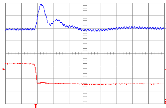
Fig. 2.5V.7: Output voltage response for V_{out} = 2.5 V to negative load current step change from 16 A to 8 A with slew rate of -5\text{ A}/\mu\text{s} at V_{in} = 5 V. Top trace: output voltage (100 mV/div.); Bottom trace: load current (5 A/div.). C_o = 100\text{ }\mu\text{F} ceramic + 1\text{ }\mu\text{F} ceramic. Time scale: 20 \mu\text{s} /div.
