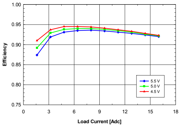
Fig. 2.5V.2: Efficiency vs. load current and input voltage for V_{out} = 2.5 V converter mounted vertically with air flowing from pin 10 to pin 1 at a rate of 200 LFM (1 m/s) and T_a = 25 °C.
