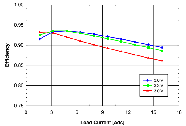
Fig. 1.8V.3: Efficiency vs. load current and input voltage for V_{out} = 1.8 V converter mounted vertically with air flowing from pin 10 to pin 1 at a rate of 200 LFM (1 m/s) and T_a = 25 °C.
