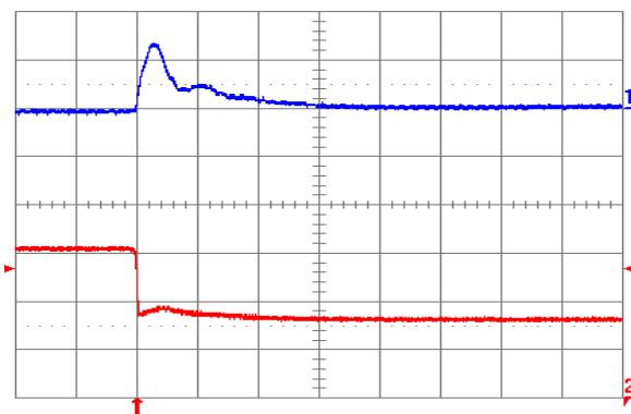
Fig. 0.7525V.7: Output voltage response for V_{out} = 0.7525 V to negative load current step change from 16 A to 8 A with slew rate of -5 A/\mu s at V_{in} = 5 V . Top trace: output voltage (100 mV/div.); Bottom trace: load current (5 A/div.). C_o = 100 \mu F ceramic + 1 \mu F ceramic. Time scale: 20 \mu s /div.
