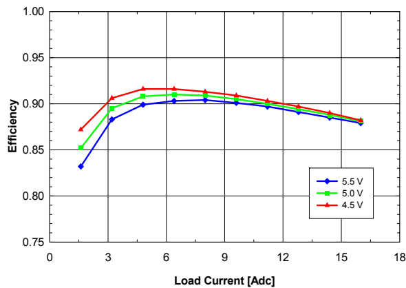
Fig. 1.5V.2: Efficiency vs. load current and input voltage for V_{out} = 1.5 V converter mounted vertically with air flowing from pin 10 to pin 1 at a rate of 200 LFM (1 m/s) and T_a = 25 °C.
