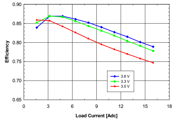
Fig. 0.7525V.3: Efficiency vs. load current and input voltage for V_{out} = 0.7525 V converter mounted vertically with air flowing from pin 10 to pin 1 at a rate of 200 LFM (1 m/s) and T_a = 25 °C.
