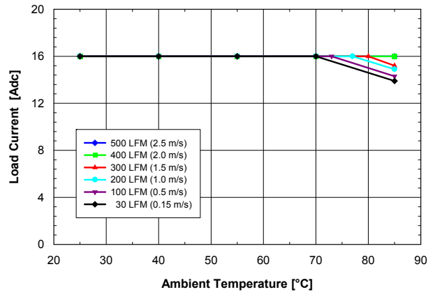
Fig. 1.8V.1: Available load current vs. ambient temperature and airflow rates for V_{out} = 1.8 V converter mounted vertically with V_{in} = 5 V, air flowing from pin 10 to pin 1, and maximum MOSFET temperature \leq 120 °C.
