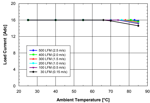
Fig. 0.7525V.1: Available load current vs. ambient temperature and airflow rates for V_{out} = 1.0 V converter mounted vertically with V_{in} = 5 V, air flowing from pin 10 to pin 1, and maximum MOSFET temperature \leq 120 °C.
