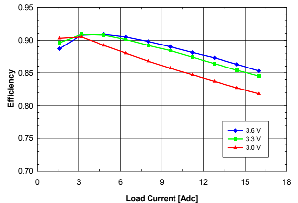
Fig. 1.2V.3: Efficiency vs. load current and input voltage for V_{out} = 1.2 V converter mounted vertically with air flowing from pin 10 to pin 1 at a rate of 200 LFM (1 m/s) and T_a = 25 °C.
