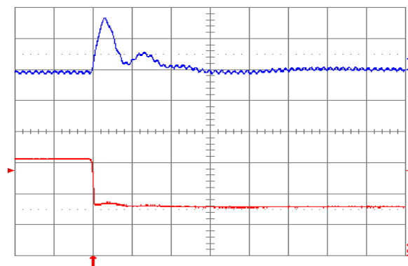
Fig. 1.8V.7: Output voltage response for V_{out} = 1.8 V to negative load current step change from 16 A to 8 A with slew rate of -5 A/ \mu s at V_{in} = 5 V. Top trace: output voltage (100 mV/div.); Bottom trace: load current (5 A/div.). C_o = 100 \mu F ceramic + 1 \mu F ceramic. Time scale: 20 \mu s/div.
