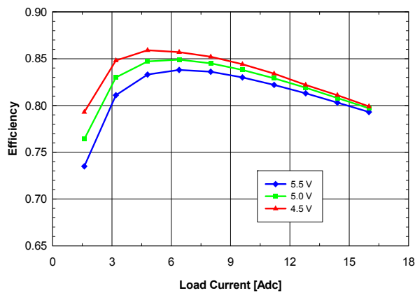
Fig. 0.7525V.2: Efficiency vs. load current and input voltage for V_{out} = 0.7525 V converter mounted vertically with air flowing from pin 10 to pin 1 at a rate of 200 LFM (1 m/s) and T_a = 25 °C.
