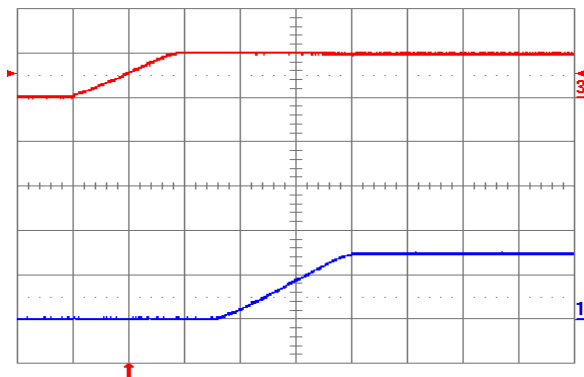
Fig. 1.5V.4: Turn-on transient for V_{out} = 1.5 V with application of V_{in} at full rated load current (resistive) and 100 \mu F external capacitance at V_{in} = 5 V. Top trace: V_{in} (5 V/div.); Bottom trace: output voltage (1 V/div.); Time scale: 2 ms/div.
