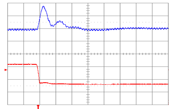
Fig. 2.0V.7: Output voltage response for V_{out} = 2.0 V to negative load current step change from 16 A to 8 A with slew rate of -5\text{ A}/\mu\text{s} at V_{in} = 5 V. Top trace: output voltage (100 mV/div.); Bottom trace: load current (5 A/div.). C_o = 100\text{ }\mu\text{F} ceramic + 1\text{ }\mu\text{F} ceramic. Time scale: 20 \mu\text{s} /div.
