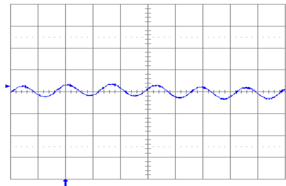
Fig. 3.3V.5: Output voltage ripple (20 mV/div.) at full rated load current into a resistive load with external capacitance 100 \mu F ceramic + 1 \mu F ceramic and V_{in} = 5 V for V_{out} = 3.3 V. Time scale: 2 \mu s/div.
