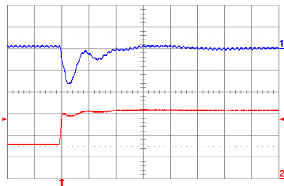
Fig. 1.8V.6: Output voltage response for V_{out} = 1.8 V to positive load current step change from 8 A to 16 A with slew rate of 5 A/ \mu s at V_{in} = 5 V. Top trace: output voltage (100 mV/div.); Bottom trace: load current (5 A/div.). C_o = 100 \mu F ceramic + 1 \mu F ceramic. Time scale: 20 \mu s/div.
