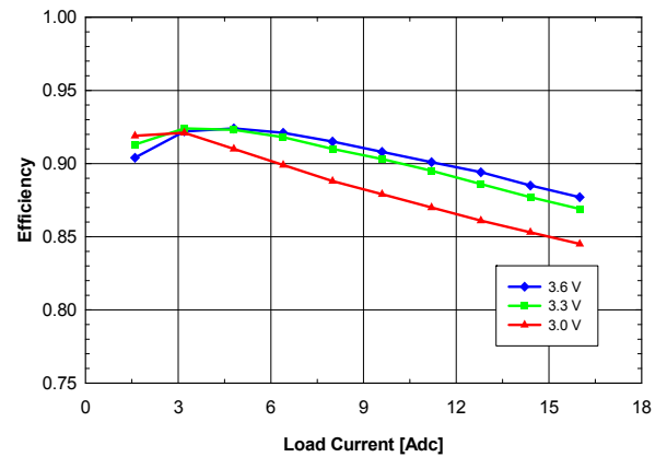
Fig. 1.5V.3: Efficiency vs. load current and input voltage for V_{out} = 1.5 V converter mounted vertically with air flowing from pin 10 to pin 1 at a rate of 200 LFM (1 m/s) and T_a = 25 °C.
