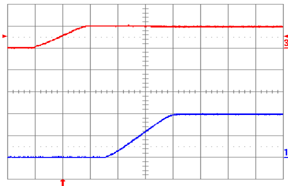
Fig. 2.0V.4: Turn-on transient for V_{out} = 2.0 V with application of V_{in} at full rated load current (resistive) and 100\text{ }\mu\text{F} external capacitance at V_{in} = 5 V. Top trace: V_{in} (5 V/div.); Bottom trace: output voltage (1 V/div.); Time scale: 2 ms/div.
