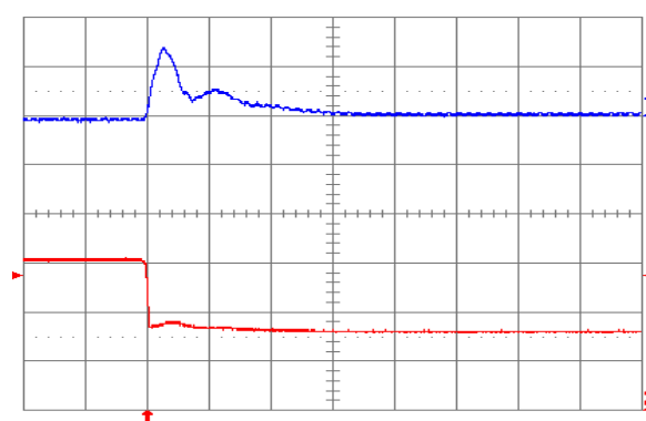
Fig. 1.0V.7: Output voltage response for V_{out} = 1.0 V to negative load current step change from 16 A to 8 A with slew rate of -5 A/ \mu s at V_{in} = 5 V. Top trace: output voltage (100 mV/div.); Bottom trace: load current (5 A/div.). C_o = 100 \mu F ceramic + 1 \mu F ceramic. Time scale: 20 \mu s/div.
