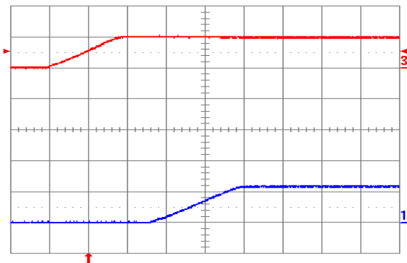
Fig. 1.2V.4: Turn-on transient for V_{out} = 1.2 V with application of V_{in} at full rated load current (resistive) and 100 \mu F external capacitance at V_{in} = 5 V. Top trace: V_{in} (5 V/div.); Bottom trace: output voltage (1 V/div.); Time scale: 2 ms/div.
