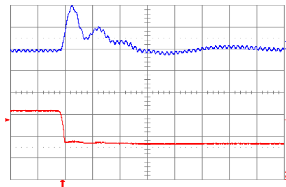
Fig. 3.3V.7: Output voltage response for V_{out} = 3.3 V to negative load current step change from 16 A to 8 A with slew rate of -5 A/ \mu s at V_{in} = 5 V. Top trace: output voltage (100 mV/div.); Bottom trace: load current (5 A/div.). C_o = 100 \mu F ceramic + 1 \mu F ceramic. Time scale: 20 \mu s/div.
