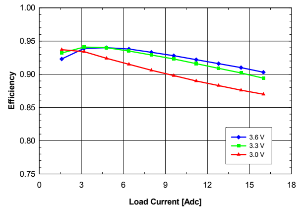
Fig. 2.0V.3: Efficiency vs. load current and input voltage for V_{out} = 2.0 V converter mounted vertically with air flowing from pin 10 to pin 1 at a rate of 200 LFM (1 m/s) and T_a = 25 °C.
