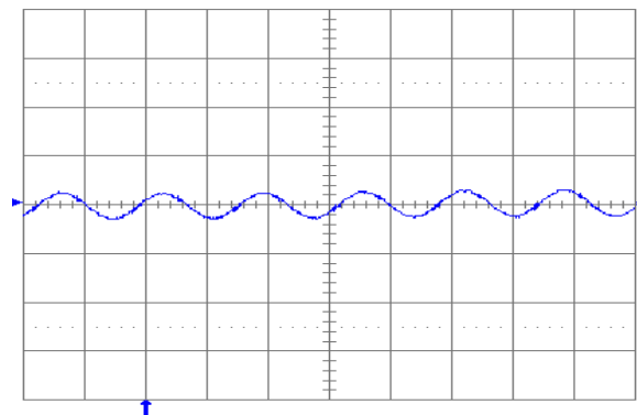
Fig. 2.5V.5: Output voltage ripple (20 mV/div.) at full rated load current into a resistive load with external capacitance 100\text{ }\mu\text{F} ceramic + 1\text{ }\mu\text{F} ceramic and V_{in} = 5 V for V_{out} = 2.5 V. Time scale: 2 \mu\text{s} /div.
