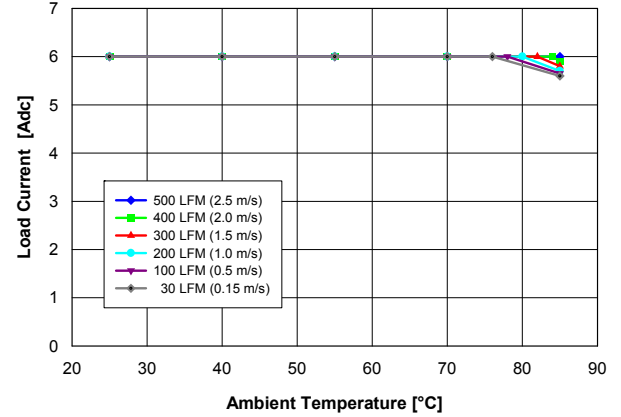
Fig. 1.5V.2: Available load current vs. ambient temperature and airflow rates for Vout = 1.5V converter mounted vertically or horizontally with Vin = 3.3V, air flowing from pin 5 to pin 1, and maximum MOSFET temperature ≤ 120°C.
