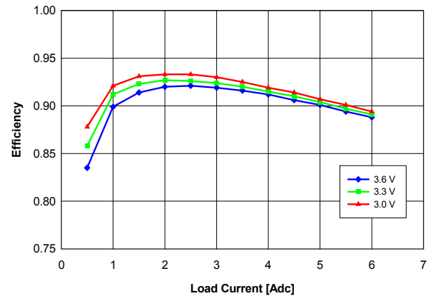
Fig. 1.8V.4: Efficiency vs. load current and input voltage for Vout = 1.8V converter mounted vertically or horizontally with air flowing from pin 5 to pin 1 at a rate of 200 LFM (1 m/s) and Ta = 25°C.
