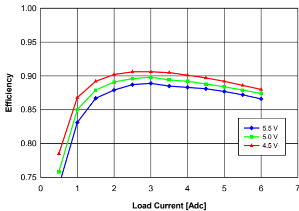
Fig. 1.8V.3: Efficiency vs. load current and input voltage for Vout = 1.8V converter mounted vertically or horizontally with air flowing from pin 5 to pin 1 at a rate of 200 LFM (1 m/s) and Ta = 25°C.
