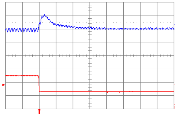
Fig. 1.2V.8: Output voltage response for V_{out} = 1.2V to negative load current step change from 5A to 2.5A with slew rate of -5A/\mu s at V_{in} = 5V . Top trace: output voltage (100mV/div.); Bottom trace: load current (2A/div.). C_o = 47\mu F ceramic. Time scale: 20\mu s /div.
