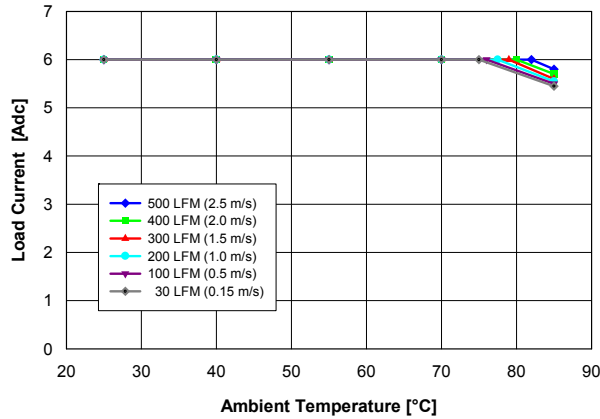
Fig. 1.8V.1: Available load current vs. ambient temperature and airflow rates for Vout = 1.8V converter mounted vertically or horizontally with Vin = 5V, air flowing from pin 5 to pin 1, and maximum MOSFET temperature ≤ 120°C.
