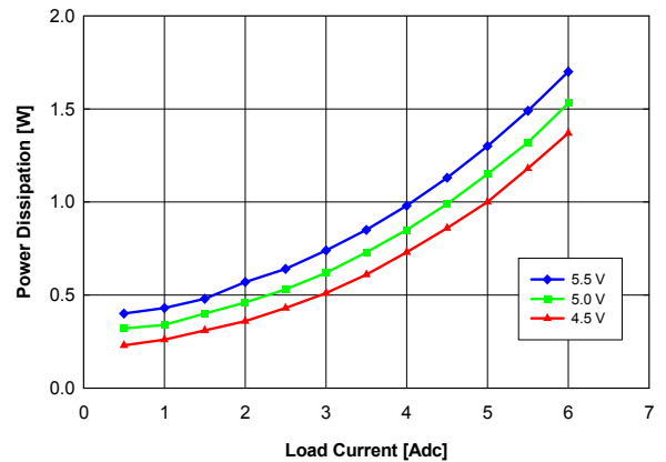
Fig. 3.3V.4: Power loss vs. load current and input voltage for V_{out} = 3.3V converter mounted vertically or horizontally with air flowing from pin 5 to pin 1 at a rate of 200 LFM (1 m/s) and T_a = 25^{\circ}C .
