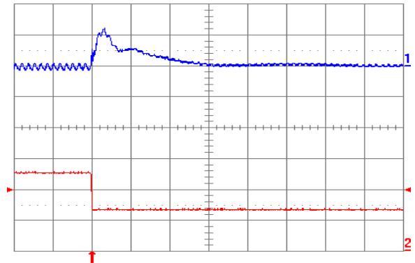
Fig. 3.3V.8: Output voltage response for V_{out} = 3.3V to negative load current step change from 5A to 2.5A with slew rate of -5A/ \mu s at V_{in} = 5V . Top trace: output voltage (100mV/div.); Bottom trace: load current (2A/div.). C_o = 47\mu F ceramic. Time scale: 20 \mu s /div.
