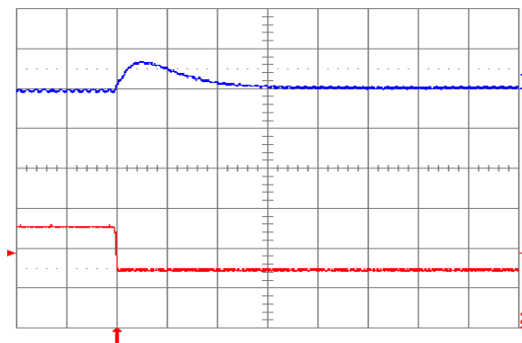
Fig. 0.7525V.8: Output voltage response for V_{out} = 0.7525V to negative load current step change from 5A to 2.5A with slew rate of -5A/\mu s at V_{in} = 5V . Top trace: output voltage (100mV/div.); Bottom trace: load current (2A/div.). C_o = 47\mu F ceramic. Time scale: 20μs/div.
