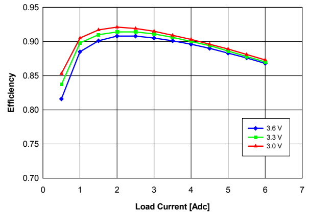
Fig. 1.5V.4: Efficiency vs. load current and input voltage for Vout = 1.5V converter mounted vertically or horizontally with air flowing from pin 5 to pin 1 at a rate of 200 LFM (1 m/s) and Ta = 25°C.
