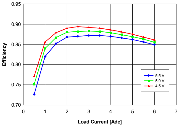
Fig. 1.5V.3: Efficiency vs. load current and input voltage for Vout = 1.5V converter mounted vertically or horizontally with air flowing from pin 5 to pin 1 at a rate of 200 LFM (1 m/s) and Ta = 25°C.
