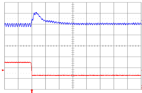
Fig. 1.5V.8: Output voltage response for V_{out} = 1.5V to negative load current step change from 5A to 2.5A with slew rate of -5A/\mu s at V_{in} = 5V . Top trace: output voltage (100mV/div.); Bottom trace: load current (2A/div.). C_o = 47\mu F ceramic. Time scale: 20\mu s /div.
