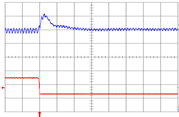
Fig. 2.0V.8: Output voltage response for V_{out} = 2.0V to negative load current step change from 5A to 2.5A with slew rate of -5A/\mu s at V_{in} = 5V . Top trace: output voltage (100mV/div.); Bottom trace: load current (2A/div.). C_o = 47\mu F ceramic. Time scale: 20\mu s /div.
