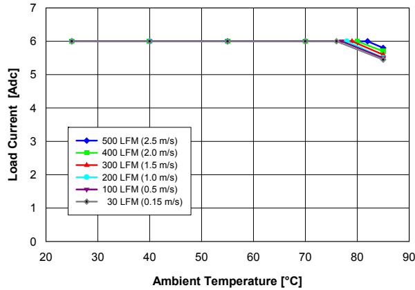
Fig. 1.5V.1: Available load current vs. ambient temperature and airflow rates for Vout = 1.5V converter mounted vertically or horizontally with Vin = 5V, air flowing from pin 5 to pin 1, and maximum MOSFET temperature ≤ 120°C.
