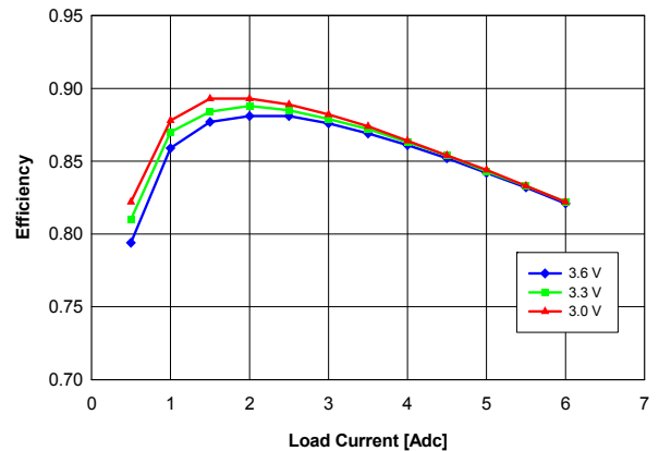
Fig. 1.0V.4: Efficiency vs. load current and input voltage for V_{out} = 1.0V converter mounted vertically or horizontally with air flowing from pin 5 to pin 1 at a rate of 200 LFM (1 m/s) and T_a = 25^{\circ}C .
