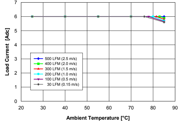
Fig. 1.8V.2: Available load current vs. ambient temperature and airflow rates for Vout = 1.8V converter mounted vertically or horizontally with Vin = 3.3V, air flowing from pin 5 to pin 1, and maximum MOSFET temperature ≤ 120°C.
