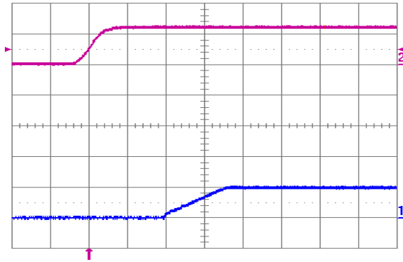
Fig. 1.0V.5: Turn-on transient for V_{out} = 1.0 V with application of V_{in} at full rated load current (resistive) and 100 \mu F external capacitance at V_{in} = 12 V. Top trace: V_{in} (10 V/div.); Bottom trace: output voltage (1 V/div.); Time scale: 2 ms/div.
