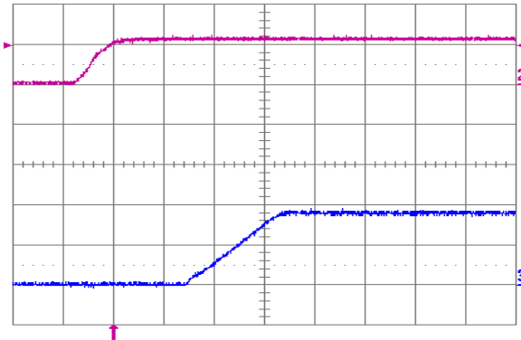
Fig. 1.8V.5: Turn-on transient for V_{out} = 1.8 V with application of V_{in} at full rated load current (resistive) and 100 \mu F external capacitance at V_{in} = 12 V. Top trace: V_{in} (10 V/div.); Bottom trace: output voltage (1 V/div.); Time scale: 2 ms/div.
