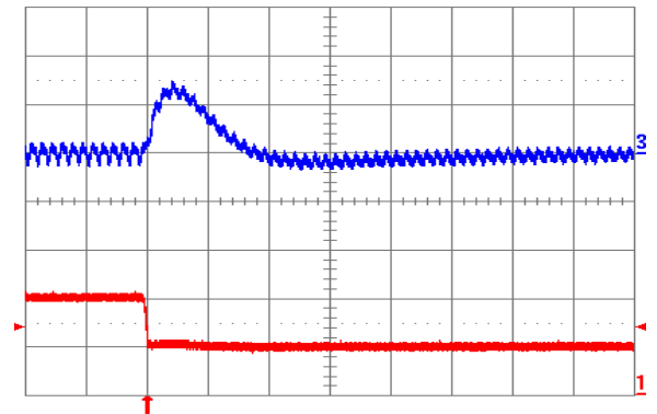
Fig. 3.3V.8: Output voltage response for V_{out} = 3.3 V to negative load current step change from 10 A to 5 A with slew rate of -5 A/ \mu s at V_{in} = 12 V. Top trace: output voltage (100 mV/div.); Bottom trace: load current (2 A/div.). C_o = 100 \mu F ceramic. Time scale: 20 \mu s/div.
