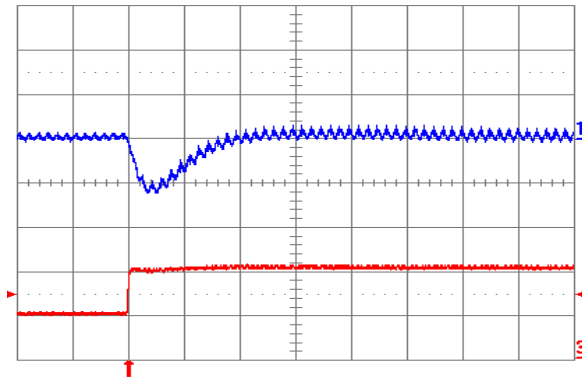
Fig. 2.0V.7: Output voltage response for V_{out} = 2.0 V to positive load current step change from 5 A to 10 A with slew rate of 5 A/ \mu s at V_{in} = 12 V. Top trace: output voltage (100 mV/div.); Bottom trace: load current (5 A/div.). C_o = 100 \mu F ceramic. Time scale: 20 \mu s/div.
