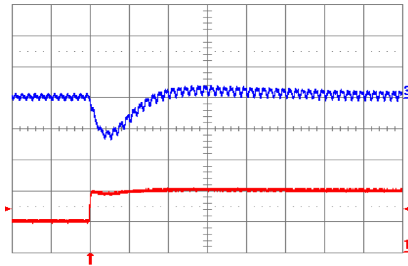
Fig. 2.5V.7: Output voltage response for V_{out} = 2.5 V to positive load current step change from 5 A to 10 A with slew rate of 5 A/ \mu s at V_{in} = 12 V. Top trace: output voltage (100 mV/div.); Bottom trace: load current (5 A/div.). C_o = 100 \mu F ceramic. Time scale: 20 \mu s/div.
