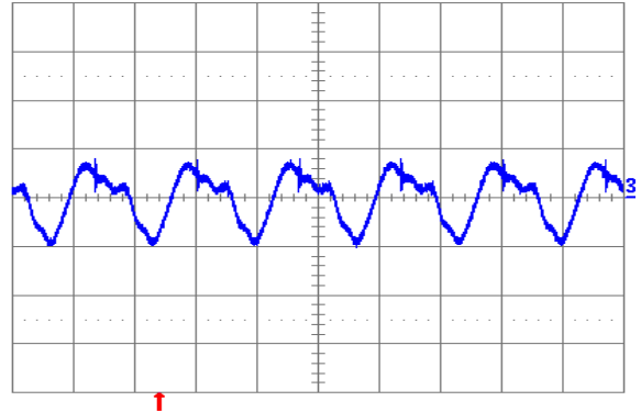
Fig. 3.3V.6: Output voltage ripple (20 mV/div.) at full rated load current into a resistive load with external capacitance 100 \mu F ceramic + 1 \mu F ceramic, and V_{in} = 12 V for V_{out} = 3.3 V. Time scale: 2 \mu s/div.
