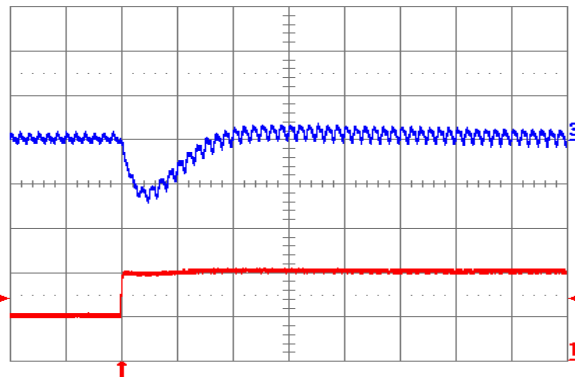
Fig. 3.3V.7: Output voltage response for V_{out} = 3.3 V to positive load current step change from 5 A to 10 A with slew rate of 5 A/ \mu s at V_{in} = 12 V. Top trace: output voltage (100 mV/div.); Bottom trace: load current (5 A/div.). C_o = 100 \mu F ceramic. Time scale: 20 \mu s/div.
