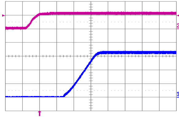
Fig. 3.3V.5: Turn-on transient for V_{out} = 3.3 V with application of V_{in} at full rated load current (resistive) and 100 \mu F external capacitance at V_{in} = 12 V. Top trace: V_{in} (10 V/div.); Bottom trace: output voltage (1 V/div.); Time scale: 2 ms/div.
