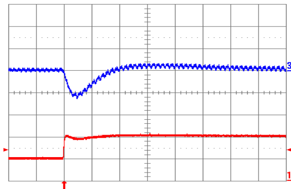
Fig. 1.2V.7: Output voltage response for V_{out} = 1.2 V to positive load current step change from 5 A to 10 A with slew rate of 5 A/ \mu s at V_{in} = 12 V. Top trace: output voltage (100 mV/div.); Bottom trace: load current (5 A/div.). C_o = 100 \mu F ceramic. Time scale: 20 \mu s/div.
