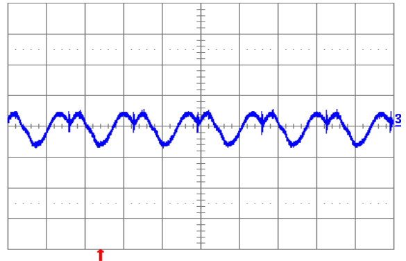
Fig. 1.8V.6: Output voltage ripple (20 mV/div.) at full rated load current into a resistive load with external capacitance 100 \mu F ceramic + 1 \mu F ceramic, and V_{in} = 12 V for V_{out} = 1.8 V. Time scale: 2 \mu s/div.
