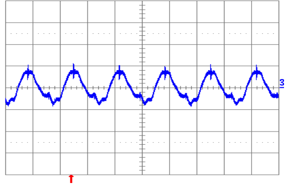
Fig. 5.0V.6: Output voltage ripple (20 mV/div.) at full rated load current into a resistive load with external capacitance 100 \mu F ceramic + 1 \mu F ceramic, and V_{in} = 12 V for V_{out} = 5.0 V. Time scale: 2 \mu s/div.
