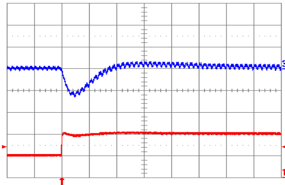
Fig. 1.5V.7: Output voltage response for V_{out} = 1.5 V to positive load current step change from 5 A to 10 A with slew rate of 5 A/ \mu s at V_{in} = 12 V. Top trace: output voltage (100 mV/div.); Bottom trace: load current (2 A/div.). C_o = 100 \mu F ceramic. Time scale: 20 \mu s/div.
