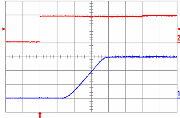
Fig. 1.5V.5: Turn-on transient for V_{out} = 1.5 V with the application of Enable signal at full rated load current (resistive) and 47 \mu F external capacitance at V_{in} = 5 V. Top trace: Enable signal (2 V/div.); Bottom trace: output voltage (500 mV/div.); Time scale: 2 ms/div.
