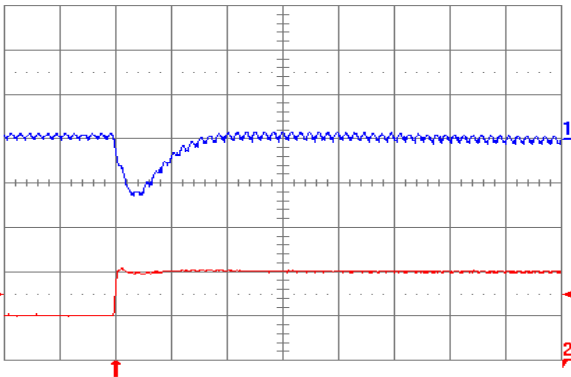
Fig. 1.2V.7: Output voltage response for V_{out} = 1.2 V to positive load current step change from 5 A to 10 A with slew rate of 5 \text{ A}/\mu\text{s} at V_{in} = 5 V. Top trace: output voltage (100 mV/div.); Bottom trace: load current (5 A/div.). C_o = 47 \mu\text{F} ceramic + 1 \mu\text{F} ceramic. Time scale: 20 \mu\text{s} /div.
