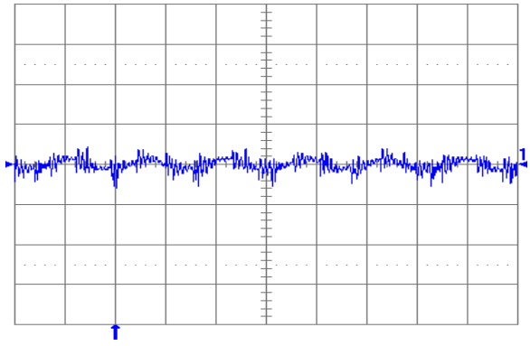
Fig. 1.5V.6: Output voltage ripple (20 mV/div.) at full rated load current into a resistive load with external capacitance 47 \mu F ceramic + 1 \mu F ceramic, and V_{in} = 5 V for V_{out} = 1.5 V. Time scale: 2 \mu s/div.
