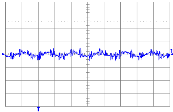
Fig. 1.8V.6: Output voltage ripple (20 mV/div.) at full rated load current into a resistive load with external capacitance 47 \mu\text{F} ceramic + 1 \mu\text{F} ceramic, and V_{in} = 5 V for V_{out} = 1.8 V. Time scale: 2 \mu\text{s} /div.
