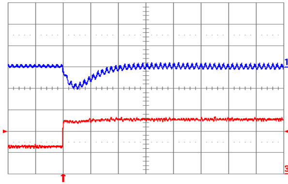
Fig. 1.0V.7: Output voltage response V_{out} = 1.0 V to positive load current step change from 5 A to 10 A with slew rate of 5 A/ \mu\text{s} at V_{in} = 5 V. Top trace: output voltage (100 mV/div.); Bottom trace: load current (5 A/div.). C_o = 47 \mu\text{F} ceramic + 1 \mu\text{F} ceramic. Time scale: 20 \mu\text{s} /div.
