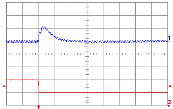
Fig. 2.5V.8: Output voltage response for V_{out} = 2.5 V to negative load current step change from 10 A to 5 A with slew rate of -5 A/ \mu\text{s} at V_{in} = 5 V. Top trace: output voltage (100 mV/div.); Bottom trace: load current (5 A/div.). C_o = 47 \mu\text{F} ceramic + 1 \mu\text{F} ceramic. Time scale: 20 \mu\text{s} /div.
