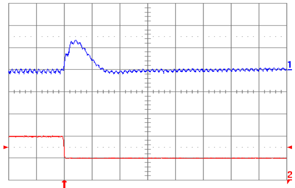
Fig. 1.2V.8: Output voltage response for V_{out} = 1.2 V to negative load current step change from 10 A to 5 A with slew rate of -5 \text{ A}/\mu\text{s} at V_{in} = 5 V. Top trace: output voltage (100 mV/div.); Bottom trace: load current (5 A/div.). C_o = 47 \mu\text{F} ceramic + 1 \mu\text{F} ceramic. Time scale: 20 \mu\text{s} /div.
