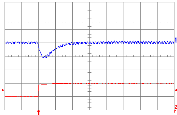
Fig. 2.0V.7: Output voltage response for V_{out} = 2.0 V to positive load current step change from 5 A to 10 A with slew rate of 5 \text{ A}/\mu\text{s} at V_{in} = 5 V. Top trace: output voltage (100 mV/div.); Bottom trace: load current (5 A/div.). C_o = 47 \mu\text{F} ceramic + 1 \mu\text{F} ceramic. Time scale: 20 \mu\text{s} /div.
