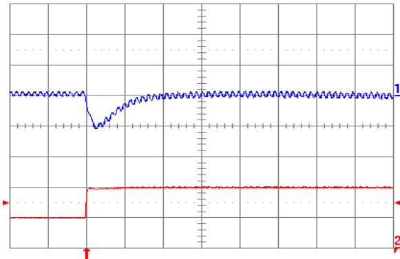
Fig. 2.5V.7: Output voltage response for V_{out} = 2.5 V to positive load current step change from 5 A to 10 A with slew rate of 5 A/ \mu\text{s} at V_{in} = 5 V. Top trace: output voltage (100 mV/div.); Bottom trace: load current (5 A/div.). C_o = 47 \mu\text{F} ceramic + 1 \mu\text{F} ceramic. Time scale: 20 \mu\text{s} /div.
