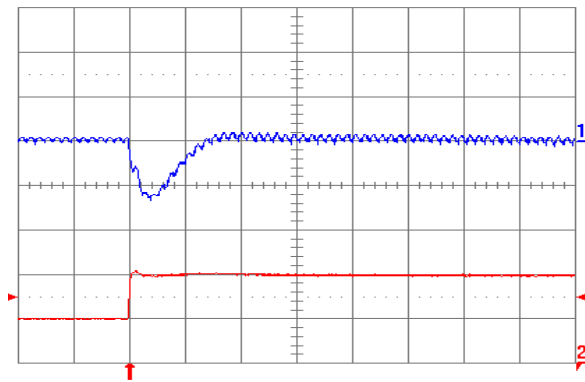
Fig. 1.5V.7: Output voltage response for V_{out} = 1.5 V to positive load current step change from 5 A to 10 A with slew rate of 5 A/ \mu s at V_{in} = 5 V. Top trace: output voltage (100 mV/div.); Bottom trace: load current (5 A/div.). C_o = 47 \mu F ceramic + 1 \mu F ceramic. Time scale: 20 \mu s/div.
