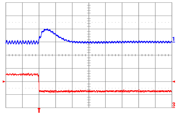
Fig. 1.0V.8: Output voltage response for V_{out} = 1.0 V to negative load current step change from 10 A to 5 A with slew rate of -5 A/ \mu\text{s} at V_{in} = 5 V. Top trace: output voltage (100 mV/div.); Bottom trace: load current (5 A/div.). C_o = 47 \mu\text{F} ceramic + 1 \mu\text{F} ceramic. Time scale: 20 \mu\text{s} /div.
