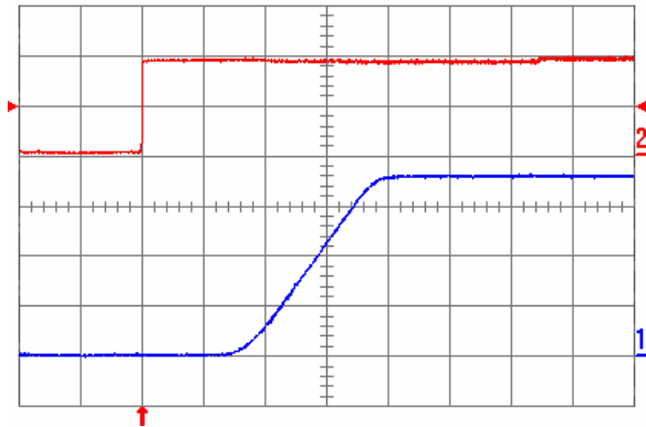
Fig. 1.8V.5: Turn-on transient for V_{out} = 1.8 V with the application of Enable signal at full rated load current (resistive) and 47 \mu\text{F} external capacitance at V_{in} = 5 V. Top trace: Enable signal (2 V/div.); Bottom trace: output voltage (500 mV/div.); Time scale: 2 ms/div.
