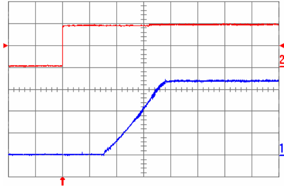
Fig. 0.7525V.5: Turn-on transient for V_{out} = 0.7525 V with the application of Enable signal at full rated load current (resistive) and 47\text{ }\mu\text{F} external capacitance at V_{in} = 5 V. Top trace: Enable signal (2 V/div.); Bottom trace: output voltage (200 mV/div.); Time scale: 2 ms/div.
