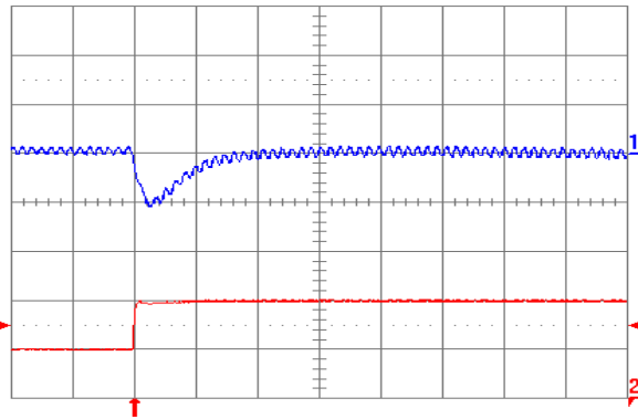
Fig. 2.5V.7: Output voltage response for V_{out} = 2.5 V to positive load current step change from 5 A to 10 A with slew rate of 5 \text{ A}/\mu\text{s} at V_{in} = 5 V. Top trace: output voltage (100 mV/div.); Bottom trace: load current (5 A/div.). C_o = 47 \mu\text{F} ceramic + 1 \mu\text{F} ceramic. Time scale: 20 \mu\text{s} /div.
