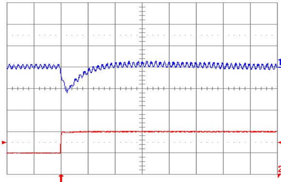
Fig. 3.3V.7: Output voltage for V_{out} = 3.3 V to positive load current step change from 5 A to 10 A with slew rate of 5\text{ A}/\mu\text{s} at V_{in} = 5 V. Top trace: output voltage (100 mV/div.); Bottom trace: load current (5 A/div.). C_o = 47\text{ }\mu\text{F} ceramic + 1\text{ }\mu\text{F} ceramic. Time scale: 20 \mu\text{s} /div.
