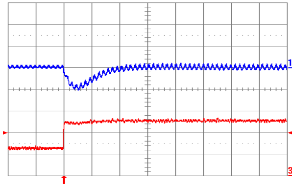
Fig. 1.0V.7: Output voltage response V_{out} = 1.0\text{ V} to positive load current step change from 5\text{ A} to 10\text{ A} with slew rate of 5\text{ A}/\mu\text{s} at V_{in} = 5\text{ V} . Top trace: output voltage ( 100\text{ mV/div.} ); Bottom trace: load current ( 5\text{ A/div.} ). C_o = 47\text{ }\mu\text{F} ceramic + 1\text{ }\mu\text{F} ceramic. Time scale: 20\text{ }\mu\text{s/div.}
