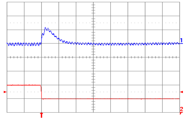
Fig. 2.5V.8: Output voltage response for V_{out} = 2.5 V to negative load current step change from 10 A to 5 A with slew rate of -5 \text{ A}/\mu\text{s} at V_{in} = 5 V. Top trace: output voltage (100 mV/div.); Bottom trace: load current (5 A/div.). C_o = 47 \mu\text{F} ceramic + 1 \mu\text{F} ceramic. Time scale: 20 \mu\text{s} /div.
