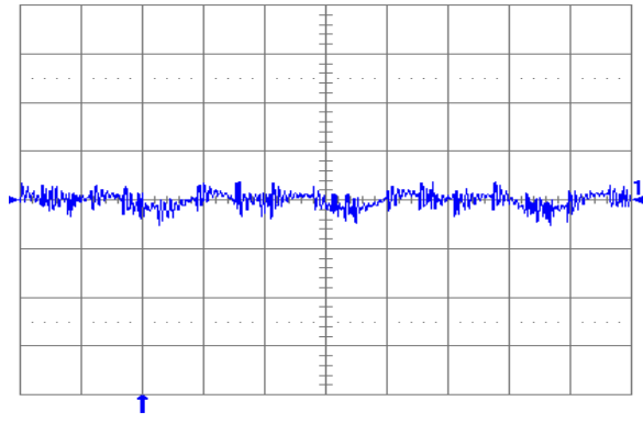
Fig. 1.0V.6: Output voltage ripple ( 20\text{ mV/div.} ) at full rated load current into a resistive load with external capacitance 47\text{ }\mu\text{F} ceramic + 1\text{ }\mu\text{F} ceramic, and V_{in} = 5\text{ V} for V_{out} = 1.0\text{ V} . Time scale: 2\text{ }\mu\text{s/div.}
