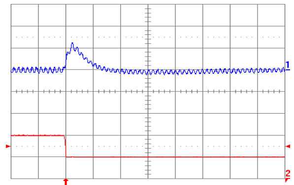
Fig. 3.3V.8: Output voltage response for V_{out} = 3.3 V to negative load current step change from 10 A to 5 A with slew rate of -5\text{ A}/\mu\text{s} at V_{in} = 5 V. Top trace: output voltage (100 mV/div.); Bottom trace: load current (5 A/div.). C_o = 47\text{ }\mu\text{F} ceramic + 1\text{ }\mu\text{F} ceramic. Time scale: 20 \mu\text{s} /div.
