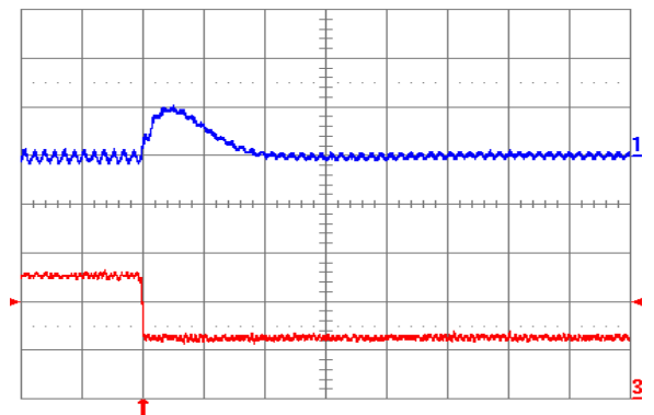
Fig. 1.0V.8: Output voltage response for V_{out} = 1.0\text{ V} to negative load current step change from 10\text{ A} to 5\text{ A} with slew rate of -5\text{ A}/\mu\text{s} at V_{in} = 5\text{ V} . Top trace: output voltage ( 100\text{ mV/div.} ); Bottom trace: load current ( 5\text{ A/div.} ). C_o = 47\text{ }\mu\text{F} ceramic + 1\text{ }\mu\text{F} ceramic. Time scale: 20\text{ }\mu\text{s/div.}
