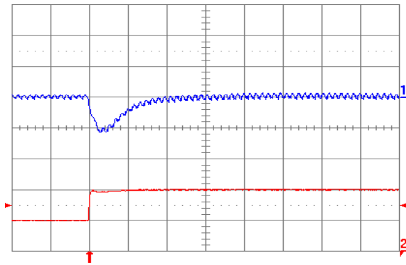
Fig. 1.8V.7: Output voltage response for V_{out} = 1.8 V to positive load current step change from 5 A to 10 A with slew rate of 5 A/ \mu s at V_{in} = 5 V. Top trace: output voltage (100 mV/div.); Bottom trace: load current (5 A/div.). C_o = 47 \mu F ceramic + 1 \mu F ceramic. Time scale: 20 \mu s/div.
