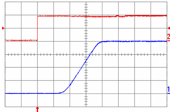
Fig. 2.0V.5: Turn-on transient for V_{out} = 2.0 V with the application of Enable signal at full rated load current (resistive) and 47\ \mu\text{F} external capacitance at V_{in} = 5 V. Top trace: Enable signal (2 V/div.); Bottom trace: output voltage (500 mV/div.); Time scale: 2 ms/div.
