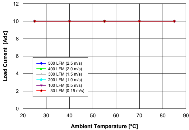
Fig. 1.2V.1: Available load current vs. ambient temperature and airflow rates for V_{out} = 1.2 V converter mounted vertically with V_{in} = 5 V, and maximum MOSFET temperature \leq 120 °C.
