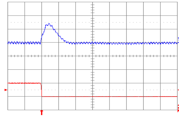
Fig. 1.8V.8: Output voltage response for V_{out} = 1.8 V to negative load current step change from 10 A to 5 A with slew rate of -5 A/ \mu s at V_{in} = 5 V. Top trace: output voltage (100 mV/div.); Bottom trace: load current (5 A/div.). C_o = 47 \mu F ceramic + 1 \mu F ceramic. Time scale: 20 \mu s/div.
