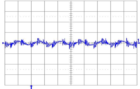
Fig. 2.0V.6: Output voltage ripple (20 mV/div.) at full rated load current into a resistive load with external capacitance 47\ \mu\text{F} ceramic + 1\ \mu\text{F} ceramic, and V_{in} = 5 V for V_{out} = 2.0 V. Time scale: 2 \mu\text{s}/\text{div} .
