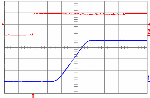
Fig. 1.8V.5: Turn-on transient for V_{out} = 1.8 V with the application of Enable signal at full rated load current (resistive) and 47 \mu F external capacitance at V_{in} = 5 V. Top trace: Enable signal (2 V/div.); Bottom trace: output voltage (500 mV/div.); Time scale: 2 ms/div.
