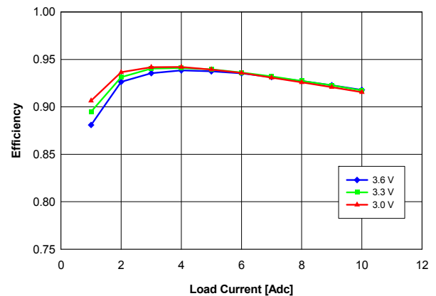
Fig. 1.8V.4: Efficiency vs. load current and input voltage for V_{out} = 1.8 V converter mounted horizontally with air flowing at a rate of 200 LFM (1 m/s) and T_a = 25 °C.
