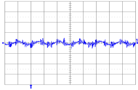
Fig. 1.8V.6: Output voltage ripple (20 mV/div.) at full rated load current into a resistive load with external capacitance 47 \mu F ceramic + 1 \mu F ceramic, and V_{in} = 5 V for V_{out} = 1.8 V. Time scale: 2 \mu s/div.
