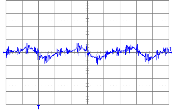
Fig. 2.5V.6: Output voltage ripple (20 mV/div.) at full rated load current into a resistive load with external capacitance 47 \mu\text{F} ceramic + 1 \mu\text{F} ceramic, and V_{in} = 5 V for V_{out} = 2.5 V. Time scale: 2 \mu\text{s} /div.
