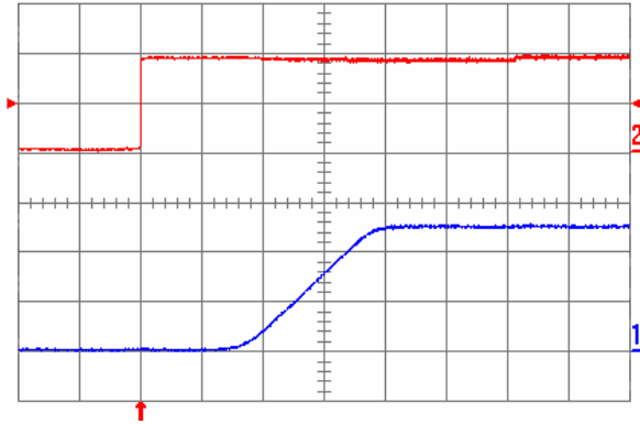
Fig. 2.5V.5: Turn-on transient for V_{out} = 2.5 V with the application of Enable signal at full rated load current (resistive) and 47 \mu\text{F} external capacitance at V_{in} = 5 V. Top trace: Enable signal (2 V/div.); Bottom trace: output voltage (1 V/div.); Time scale: 2 ms/div.
