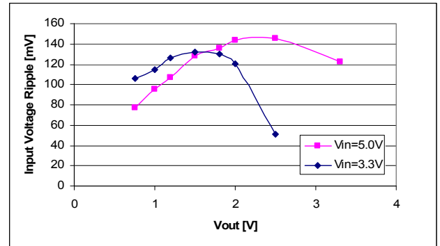
Fig. B: Input Voltage Ripple, C_{IN} = 470 \mu\text{F} polymer + 2 x 47 \mu\text{F} ceramic.
