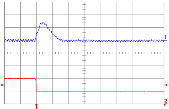
Fig. 1.8V.8: Output voltage response (YNL05S10018) to negative load current step change from 10 A to 5 A with slew rate of -5 A/ \mu s at V_{in} = 5 V. Top trace: output voltage (100 mV/div.); Bottom trace: load current (5 A/div.). C_o = 47 \mu F ceramic + 1 \mu F ceramic. Time scale: 20 \mu s/div.
