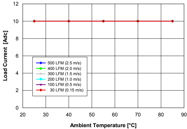
Fig. 2.5V.1: Available load current vs. ambient temperature and airflow rates for YNL05S10025 converter mounted vertically with V_{in} = 5 V, and maximum MOSFET temperature \leq 110 °C.
