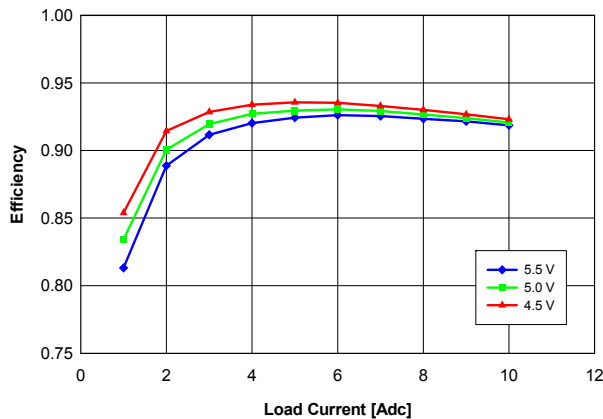
Fig. 2.0V.3: Efficiency vs. load current and input voltage for YNL05S10020 converter mounted vertically with air flowing at a rate of 200 LFM (1 m/s) and T_a = 25 °C.
