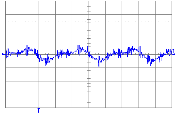
Fig. 2.5V.6: Output voltage ripple (20 mV/div.) at full rated load current into a resistive load with external capacitance 47 \mu F ceramic + 1 \mu F ceramic and V_{in} = 5 V (YNL05S10025). Time scale: 2 \mu s/div.
