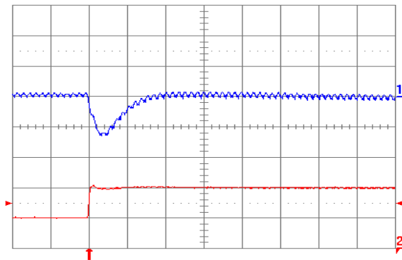
Fig. 1.2V.7: Output voltage response (YNL05S10012) to positive load current step change from 5 A to 10 A with slew rate of 5 A/ \mu s at V_{in} = 5 V. Top trace: output voltage (100 mV/div.); Bottom trace: load current (5 A/div.). C_o = 47 \mu F ceramic + 1 \mu F ceramic. Time scale: 20 \mu s/div.
