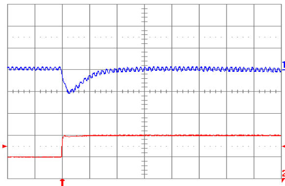
Fig. 2.5V.7: Output voltage response (YNL05S10025) to positive load current step change from 5 A to 10 A with slew rate of 5 A/ \mu s at V_{in} = 5 V. Top trace: output voltage (100 mV/div.); Bottom trace: load current (5 A/div.). C_o = 47 \mu F ceramic + 1 \mu F ceramic. Time scale: 20 \mu s/div.
