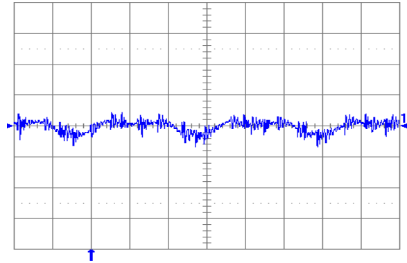
Fig. 1.2V.6: Output voltage ripple (20 mV/div.) at full rated load current into a resistive load with external capacitance 47 \mu F ceramic + 1 \mu F ceramic and V_{in} = 5 V (YNL05S10012). Time scale: 2 \mu s/div.
