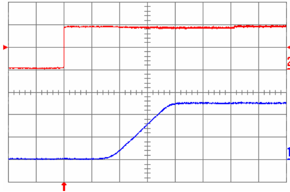
Fig. 2.5V.5: Turn-on transient (YNL05S10025) with the application of Enable signal at full rated load current (resistive) and 47 \mu F external capacitance at V_{in} = 5 V. Top trace: Enable signal (2 V/div.); Bottom trace: output voltage (1 V/div.); Time scale: 2 ms/div.
