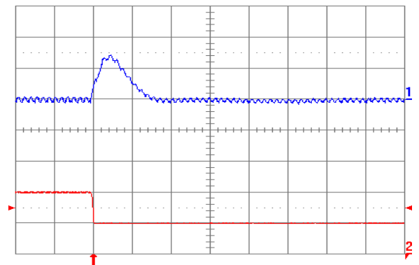
Fig. 2.0V.8: Output voltage response (YNL05S10020) to negative load current step change from 10 A to 5 A with slew rate of -5 A/ \mu s at V_{in} = 5 V. Top trace: output voltage (100 mV/div.); Bottom trace: load current (5 A/div.). C_o = 47 \mu F ceramic + 1 \mu F ceramic. Time scale: 20 \mu s/div.
