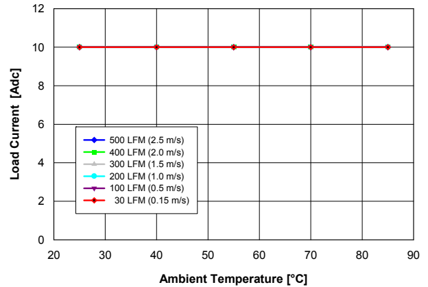
Fig. 1.5V.2: Available load current vs. ambient temperature and airflow rates for YNL05S10015 converter mounted horizontally with V_{in} = 5 V, and maximum MOSFET temperature \leq 110 °C.
