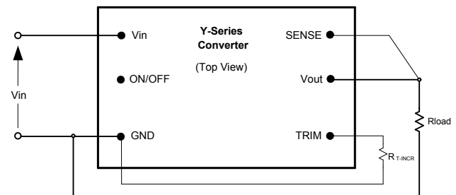
Fig. E: Configuration for increasing output voltage.
