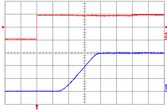
Fig. 1.5V.5: Turn-on transient (YNL05S10015) with the application of Enable signal at full rated load current (resistive) and 47 \mu F external capacitance at V_{in} = 5 V. Top trace: Enable signal (2 V/div.); Bottom trace: output voltage (500 mV/div.); Time scale: 2 ms/div.
