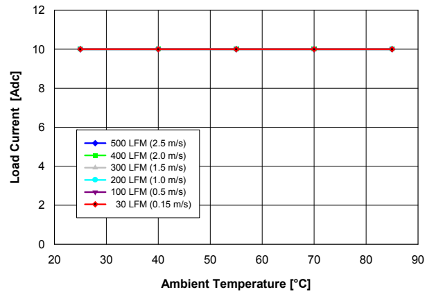
Fig. 1.8V.2: Available load current vs. ambient temperature and airflow rates for YNL05S10018 converter mounted horizontally with V_{in} = 5\text{ V} , and maximum MOSFET temperature \leq 110\text{ }^{\circ}\text{C} .
