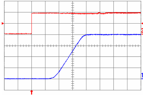
Fig. 2.0V.5: Turn-on transient (YNL05S10020) with the application of Enable signal at full rated load current (resistive) and 47 \mu F external capacitance at V_{in} = 5 V. Top trace: Enable signal (2 V/div.); Bottom trace: output voltage (500 mV/div.); Time scale: 2 ms/div.
