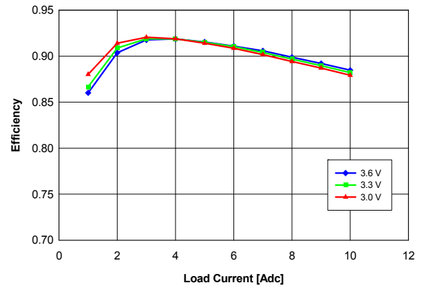
Fig. 1.2V.4: Efficiency vs. load current and input voltage for YNL05S10012 converter mounted vertically with air flowing at a rate of 200 LFM (1 m/s) and T_a = 25\text{ }^{\circ}\text{C} .
