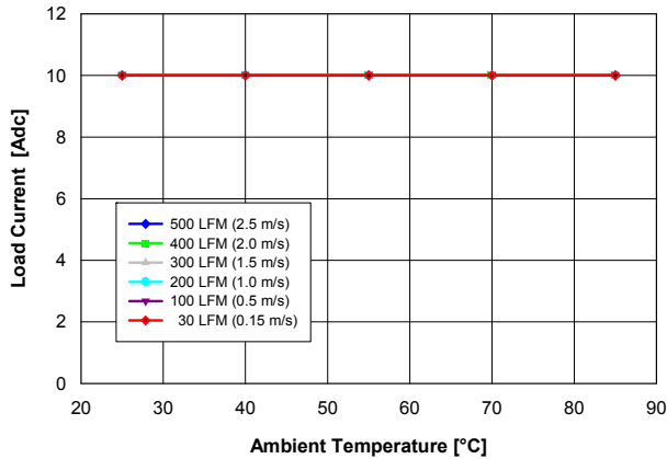
Fig. 1.0V.1: Available load current vs. ambient temperature and airflow rates YNL05S10010 converter mounted vertically with V_{in} = 5 V, and maximum MOSFET temperature \leq 110 °C.
