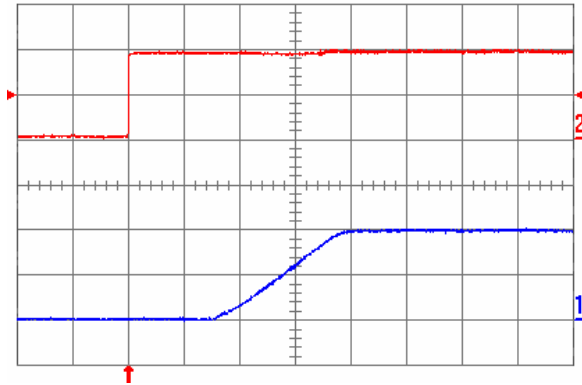
Fig. 1.0V.5: Turn-on transient (YNL05S10010) with the application of Enable signal at full rated load current (resistive) and 47 \mu F external capacitance at V_{in} = 5 V. Top trace: Enable signal (2 V/div.); Bottom trace: output voltage (500 mV/div.); Time scale: 2 ms/div.
