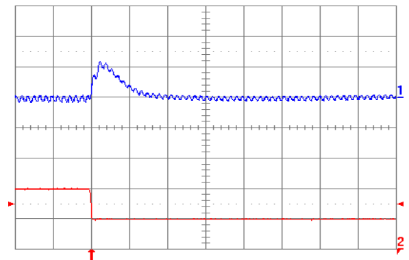
Fig. 2.5V.8: Output voltage response (YNL05S10025) to negative load current step change from 10 A to 5 A with slew rate of -5 A/ \mu s at V_{in} = 5 V. Top trace: output voltage (100 mV/div.); Bottom trace: load current (5 A/div.). C_o = 47 \mu F ceramic + 1 \mu F ceramic. Time scale: 20 \mu s/div.
