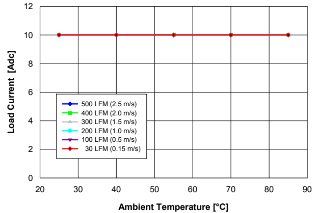
Fig. 2.5V.2: Available load current vs. ambient temperature and airflow rates for YNL05S10025 converter mounted horizontally with V_{in} = 5 V, and maximum MOSFET temperature \leq 110 °C.
