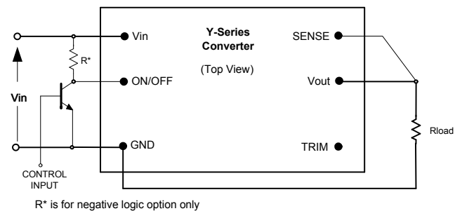
Fig. C: Circuit configuration for ON/OFF function.
