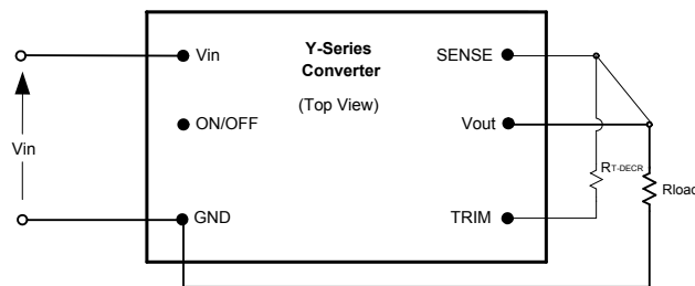
Fig. F: Configuration for decreasing output voltage.
