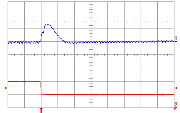
Fig. 1.2V.8: Output voltage response (YNL05S10012) to negative load current step change from 10 A to 5 A with slew rate of -5 A/ \mu s at V_{in} = 5 V. Top trace: output voltage (100 mV/div.); Bottom trace: load current (5 A/div.). C_o = 47 \mu F ceramic + 1 \mu F ceramic. Time scale: 20 \mu s/div.
