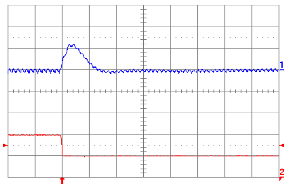
Fig. 1.5V.8: Output voltage response (YNL05S10015) to negative load current step change from 10 A to 5 A with slew rate of -5 A/ \mu s at V_{in} = 5 V. Top trace: output voltage (100 mV/div.); Bottom trace: load current (5 A/div.). C_o = 47 \mu F ceramic + 1 \mu F ceramic. Time scale: 20 \mu s/div.
