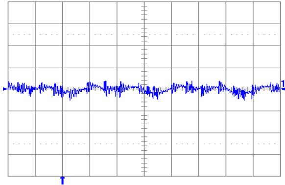
Fig. 1.0V.6: Output voltage ripple (20 mV/div.) at full rated load current into a resistive load with external capacitance 47 \mu F ceramic + 1 \mu F ceramic and V_{in} = 5 V (YNL05S10010). Time scale: 2 \mu s/div.
