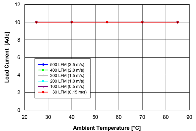
Fig. 2.0V.2: Available load current vs. ambient temperature and airflow rates for YNL05S10020 converter mounted horizontally with V_{in} = 5 V, and maximum MOSFET temperature \leq 110 °C.
