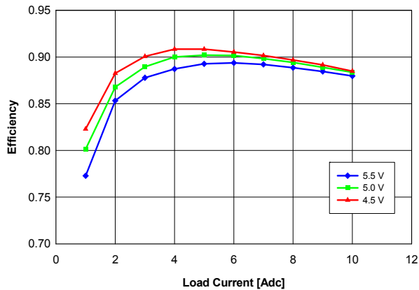
Fig. 1.2V.3: Efficiency vs. load current and input voltage for YNL05S10012 converter mounted vertically with air flowing at a rate of 200 LFM (1 m/s) and T_a = 25\text{ }^{\circ}\text{C} .
