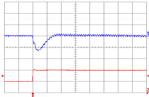
Fig. 1.5V.7: Output voltage response (YNL05S10015) to positive load current step change from 5 A to 10 A with slew rate of 5 A/ \mu s at V_{in} = 5 V. Top trace: output voltage (100 mV/div.); Bottom trace: load current (5 A/div.). C_o = 47 \mu F ceramic + 1 \mu F ceramic. Time scale: 20 \mu s/div.
