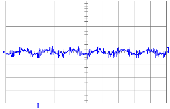
Fig. 1.8V.6: Output voltage ripple (20 mV/div.) at full rated load current into a resistive load with external capacitance 47 \mu F ceramic + 1 \mu F ceramic and V_{in} = 5 V (YNL05S10018). Time scale: 2 \mu s/div.
