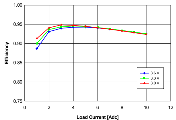
Fig. 2.0V.4: Efficiency vs. load current and input voltage for YNL05S10020 converter mounted vertically with air flowing at a rate of 200 LFM (1 m/s) and T_a = 25 °C.
