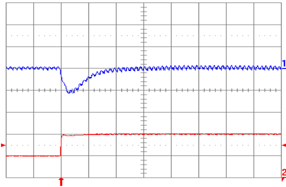
Fig. 1.8V.7: Output voltage response (YNL05S10018) to positive load current step change from 5 A to 10 A with slew rate of 5 A/ \mu s at V_{in} = 5 V. Top trace: output voltage (100 mV/div.); Bottom trace: load current (5 A/div.). C_o = 47 \mu F ceramic + 1 \mu F ceramic. Time scale: 20 \mu s/div.
