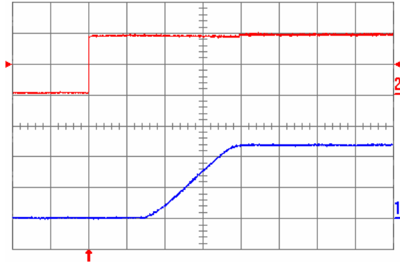
Fig. 1.2V.5: Turn-on transient (YNL05S10012) with the application of Enable signal at full rated load current (resistive) and 47 \mu F external capacitance at V_{in} = 5 V. Top trace: Enable signal (2 V/div.); Bottom trace: output voltage (500 mV/div.); Time scale: 2 ms/div.
