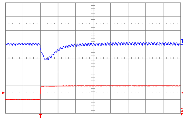
Fig. 2.0V.7: Output voltage response (YNL05S10020) to positive load current step change from 5 A to 10 A with slew rate of 5 A/ \mu s at V_{in} = 5 V. Top trace: output voltage (100 mV/div.); Bottom trace: load current (5 A/div.). C_o = 47 \mu F ceramic + 1 \mu F ceramic. Time scale: 20 \mu s/div.
