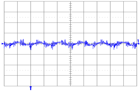
Fig. 1.5V.6: Output voltage ripple (20 mV/div.) at full rated load current into a resistive load with external capacitance 47 \mu F ceramic + 1 \mu F ceramic and V_{in} = 5 V (YNL05S10015). Time scale: 2 \mu s/div.
