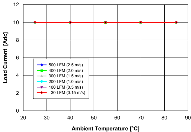
Fig. 2.0V.1: Available load current vs. ambient temperature and airflow rates for YNL05S10020 converter mounted vertically with V_{in} = 5 V, and maximum MOSFET temperature \leq 110 °C.
