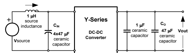
Fig. H: Test Setup for measuring input reflected-ripple currents, i_s and output voltage ripple.
