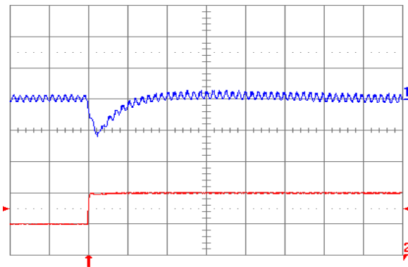
Fig. 3.3V.7: Output voltage (YNL05S10033) to positive load current step change from 5 A to 10 A with slew rate of 5 A/ \mu s at V_{in} = 5 V. Top trace: output voltage (100 mV/div.); Bottom trace: load current (5 A/div.). C_o = 47 \mu F ceramic + 1 \mu F ceramic. Time scale: 20 \mu s/div.
