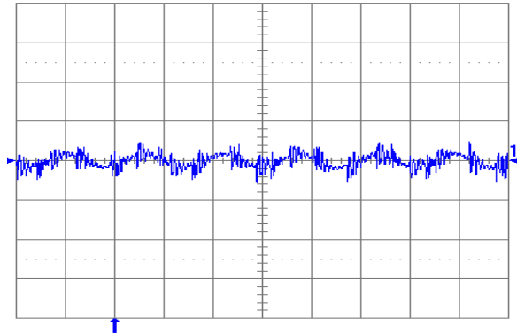
Fig. 2.0V.6: Output voltage ripple (20 mV/div.) at full rated load current into a resistive load with external capacitance 47 \mu F ceramic + 1 \mu F ceramic and V_{in} = 5 V (YNL05S10020). Time scale: 2 \mu s/div.
