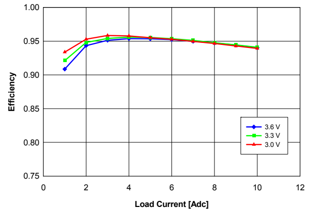
Fig. 2.5V.4: Efficiency vs. load current and input voltage for YNL05S10025 converter mounted horizontally with air flowing at a rate of 200 LFM (1 m/s) and T_a = 25 °C.
