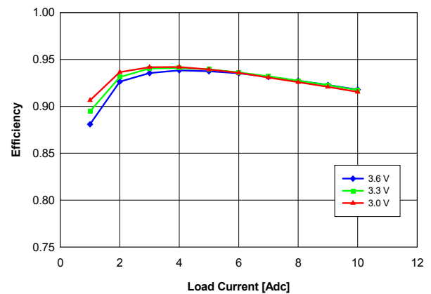
Fig. 1.8V.4: Efficiency vs. load current and input voltage for YNL05S10018 converter mounted vertically with air flowing at a rate of 200 LFM (1 m/s) and T_a = 25\text{ }^{\circ}\text{C} .
