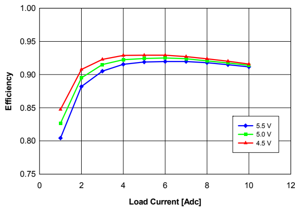
Fig. 1.8V.3: Efficiency vs. load current and input voltage for YNL05S10018 converter mounted vertically with air flowing at a rate of 200 LFM (1 m/s) and T_a = 25\text{ }^{\circ}\text{C} .
