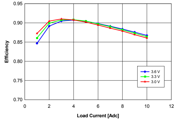
Fig. 1.0V.4: Efficiency vs. load current and input voltage for YNL05S10010 converter mounted horizontally with air flowing at a rate of 200 LFM (1 m/s) and T_a = 25 °C.
