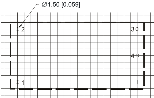
PCB LAYOUT
