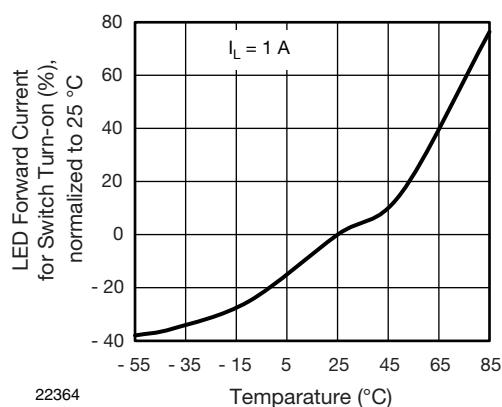
Fig. 7 - LED Current for Switch Turn-on vs. Temperature
