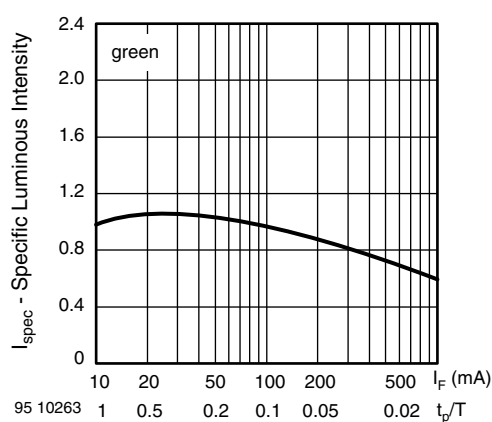
Fig. 6 - Specific Luminous Intensity vs. Forward Current
