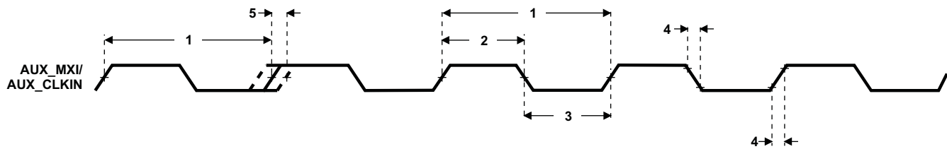
Figure 6-16. AUX_MXI/AUX_CLKIN Timing
