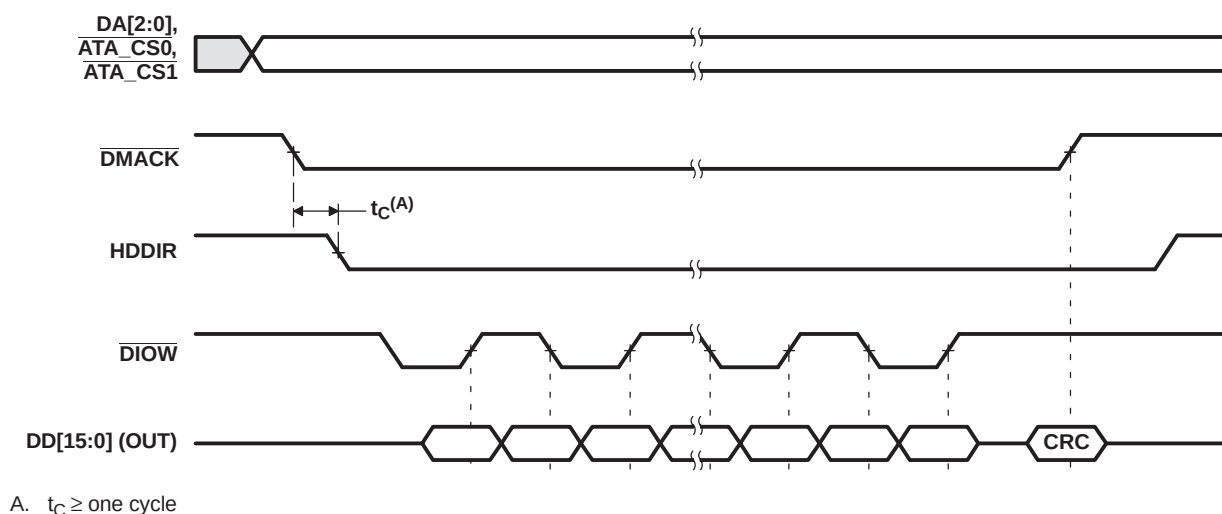
Figure 6-79. ATA HDDIR Ultra DMA Write Transfer Timing
