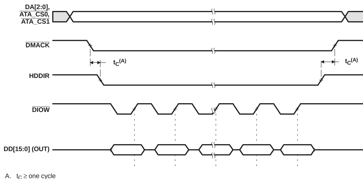
Figure 6-78. ATA HDDIR Multiword DMA Write Transfer Timing
