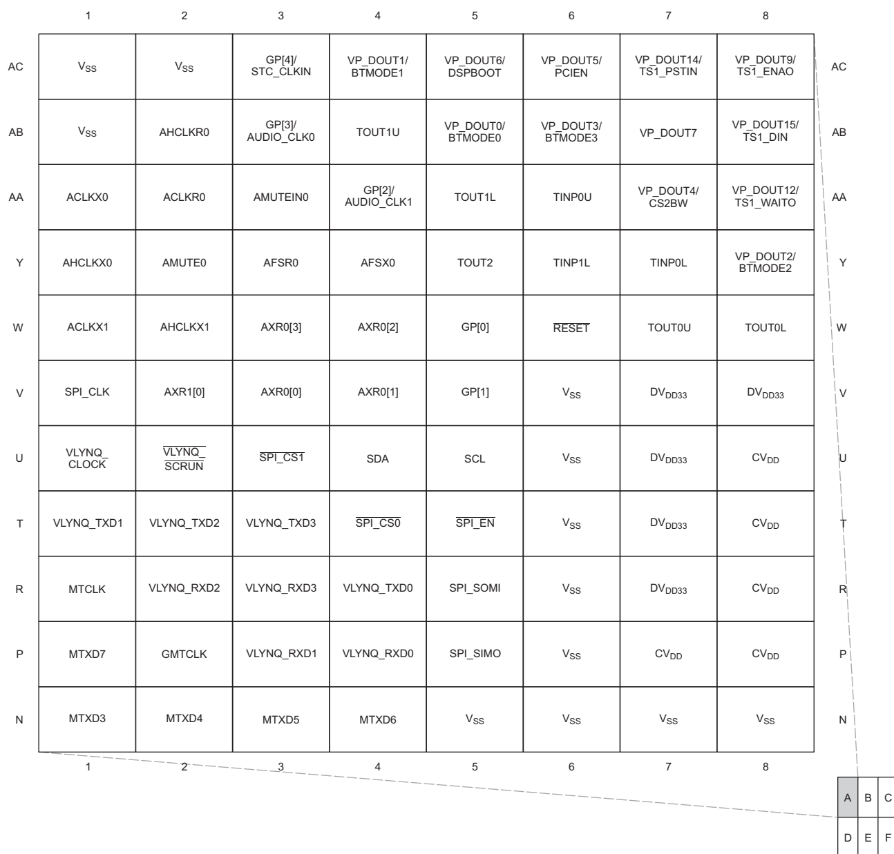
Figure 2-3. Pin Map [Section A]
