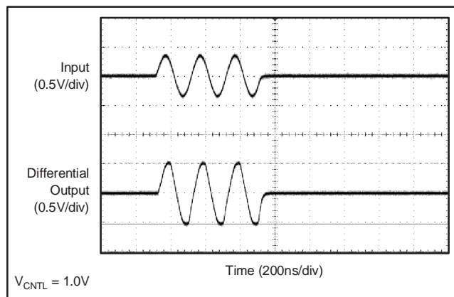
Figure 41. Approaching Overload (700mV pp Input)
