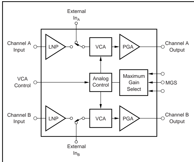
FIGURE 1. Simplified Block Diagram of the VCA2613.
