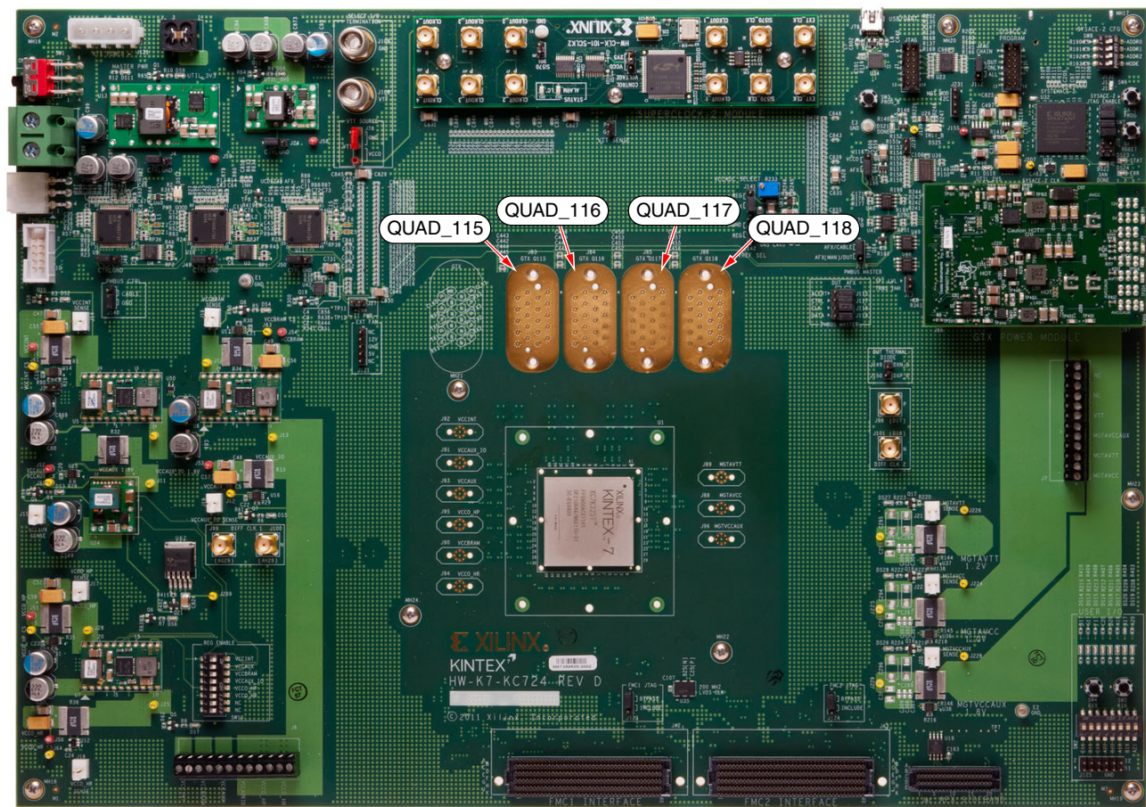
Figure 1-13: GTX Quad Locations
