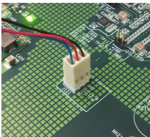
Figure 1-9: Heatsink Fan Power Connector J121
