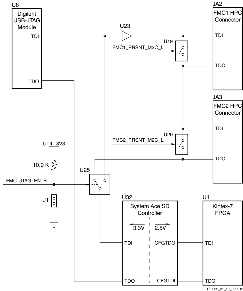
Figure 1-10: JTAG Chain
