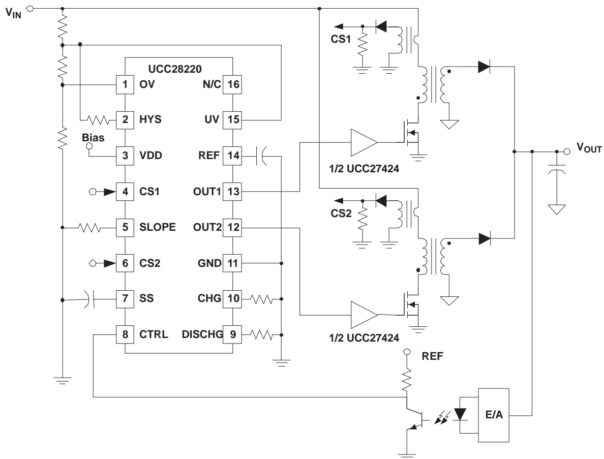
Figure 4. Interleaved Flyback Application Circuit
