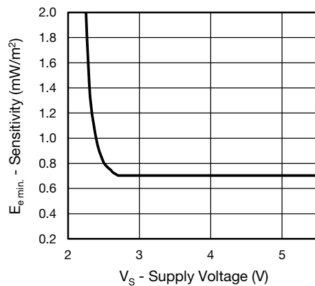
Fig. 11 - Sensitivity vs. Supply Voltage
