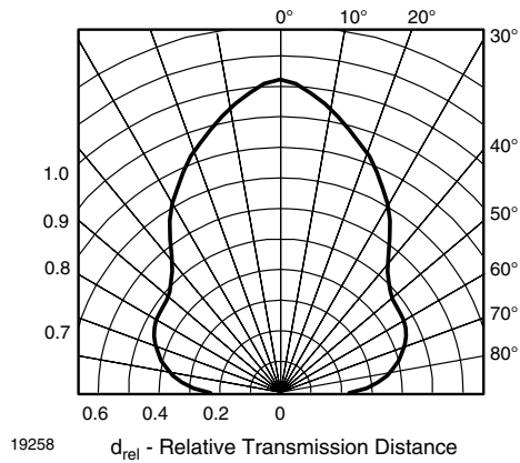
Fig. 9 - Horizontal Directivity
