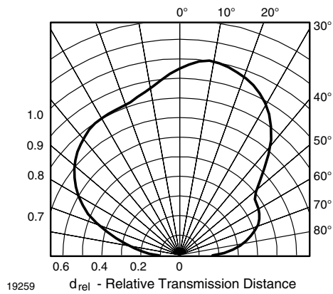
Fig. 10 - Vertical Directivity
