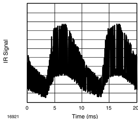
Fig. 15 - IR Distrubance from Fluorescent Lamp with High Modulation
