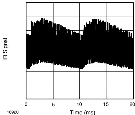
Fig. 14 - IR Distrubance from Fluorescent Lamp with Low Modulation
