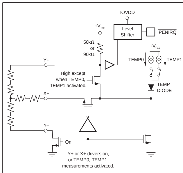
Figure 10. PENIRO Functional Block Diagram
