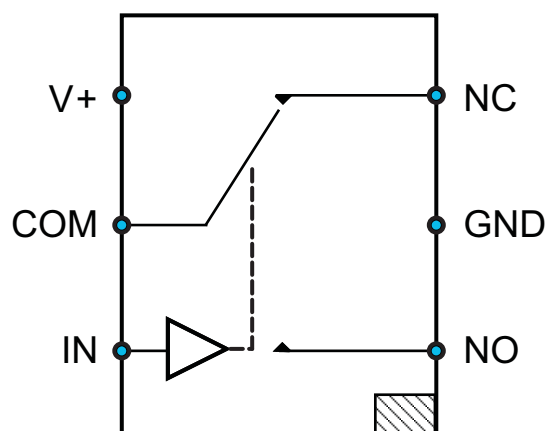
Figure 1. Logic Diagram
