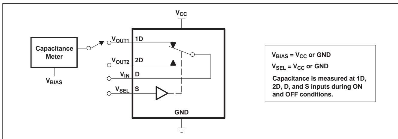
Figure 16. Capacitance
