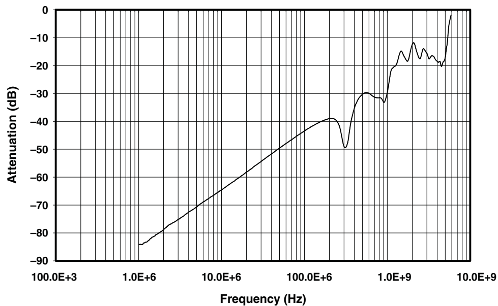
Figure 2. OFF Isolation
