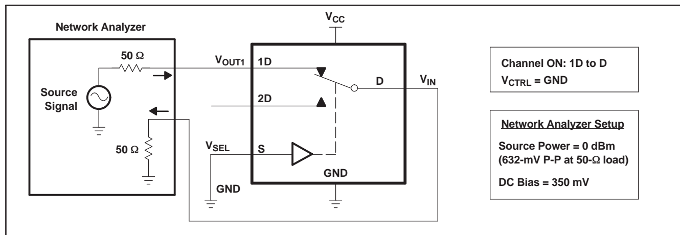
Figure 11. Bandwidth (BW)
