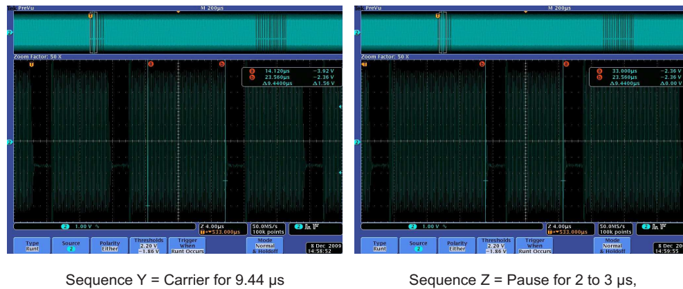
Figure 5-30. Receive Data Bits and Framing Level
