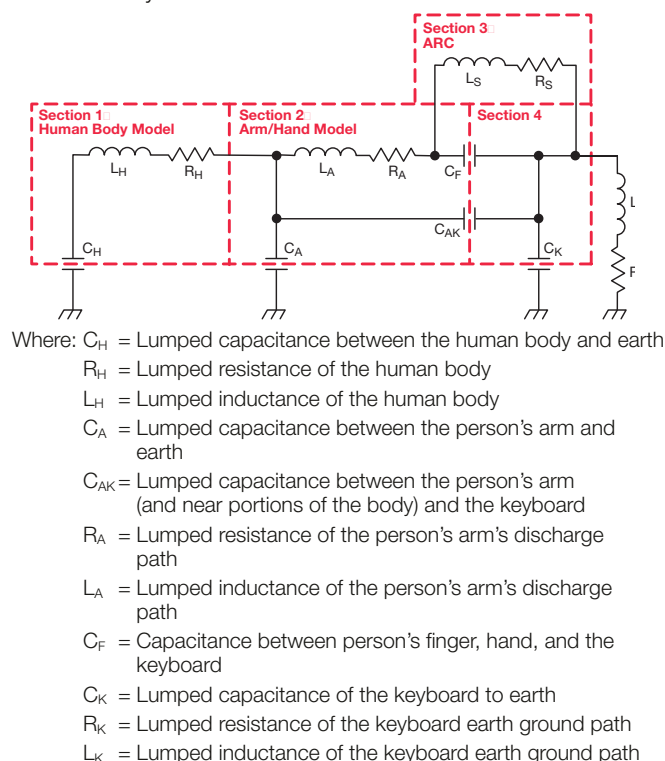
Figure 4. Contact Discharge Model
