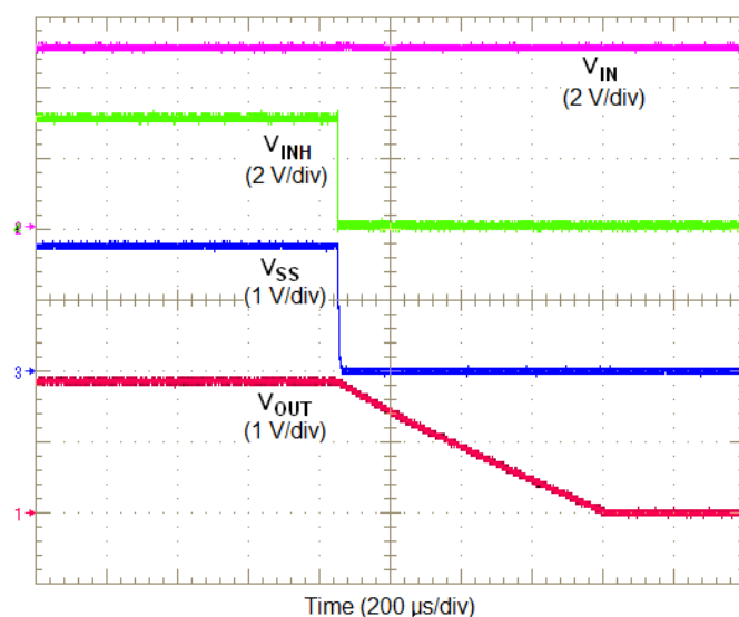
Figure 30. Inhibit Turn-Off
