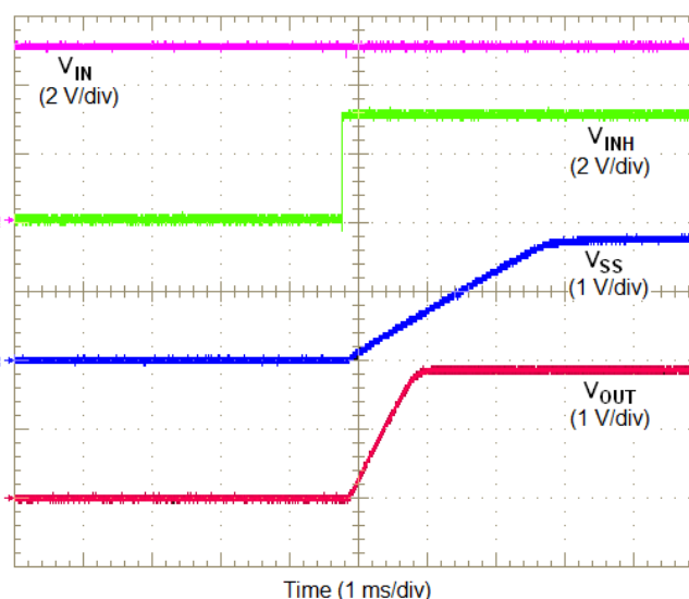
Figure 31. Inhibit Turn-On
