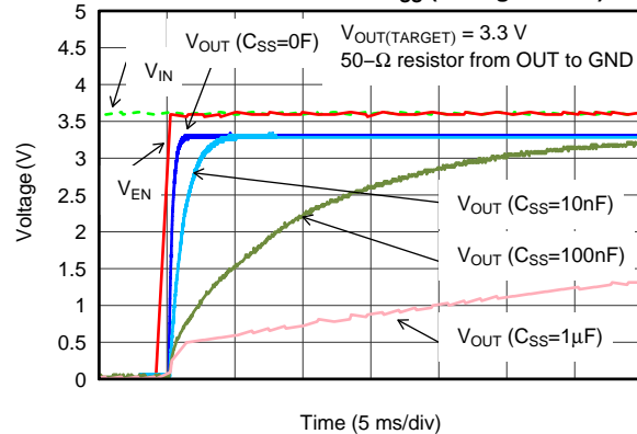
SOFT-START DELAY vs C_{SS} (Enlarged View)
