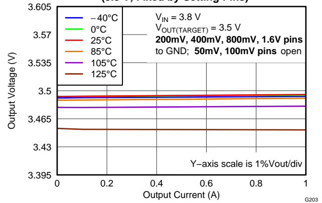
LOAD REGULATION (3.5 V, Fixed by Setting Pins)
