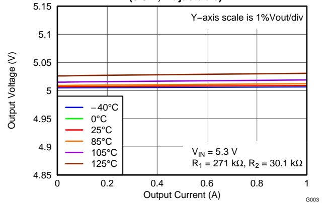
LOAD REGULATION (5.0 V, Adjustable)
