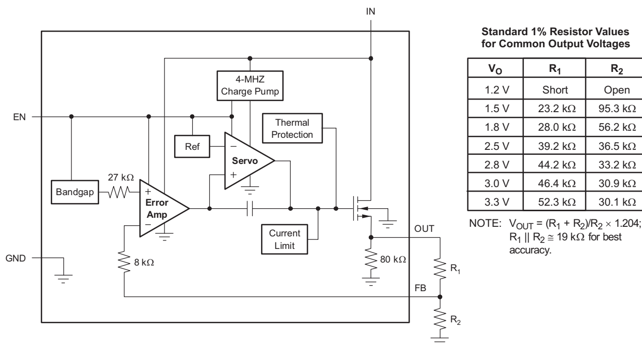
Figure 2. Adjustable Voltage Version (Product-Preview Device)
