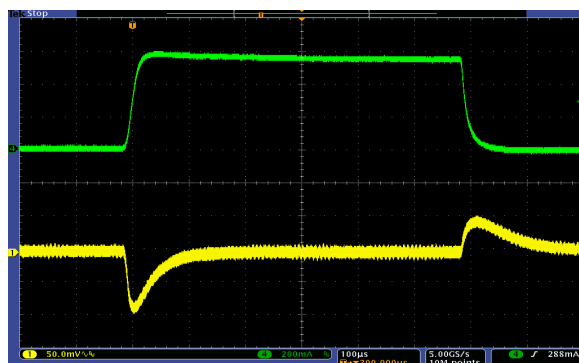
Figure 13. Load Transient Response, 10 mA to 550 mA
