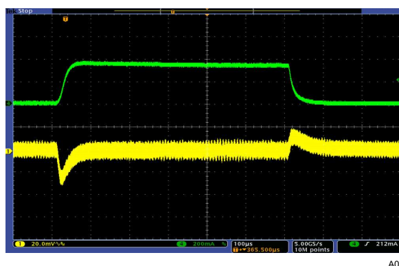
Figure 16. Load Transient Response, 10 mA to 350 mA
