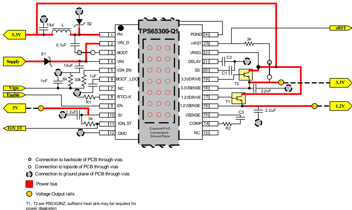
Figure 23. PCB Layout
