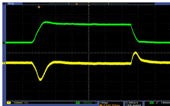
Figure 10. Load Transient Response, 10 mA to 200 mA
