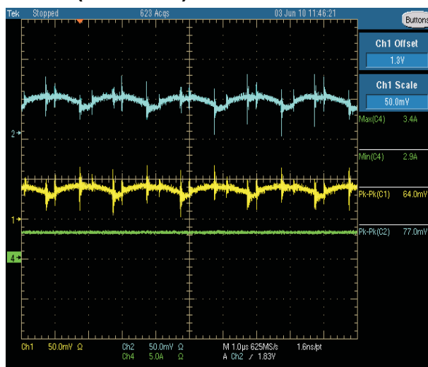
Figure 10. Ripple for Buck 1 (Yellow Trace) 1.2 V, 3 A and Buck 2 (Blue Trace) 1.8 V, 2 A, 50 mV per Division V_{IN} = 12 V, f_{SW} = 500 kHz, L_O = 4.7 \mu H, DCR = 10 m \Omega , C_O = 22 \mu F
