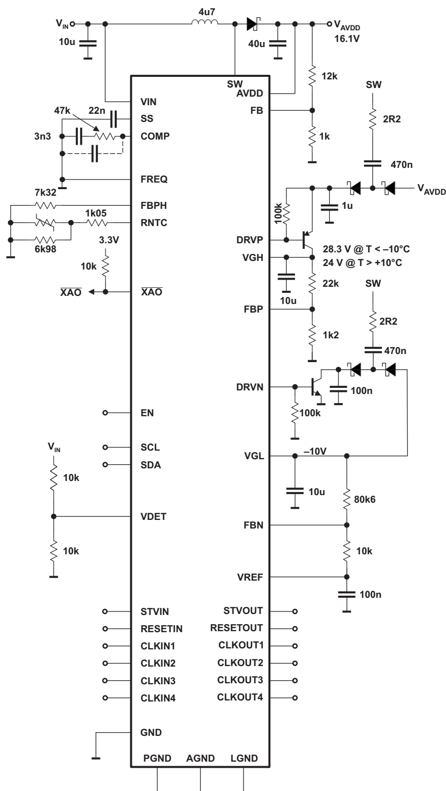
Figure 39. Typical Application Circuit Using Positive Charge Pump in \times 2 Configuration
