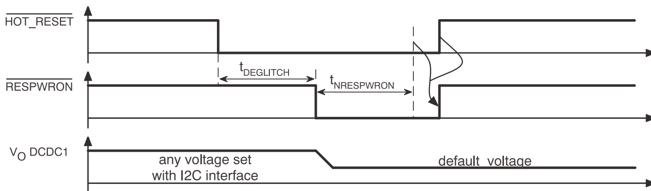
Figure 27. HOT_RESET Timing
