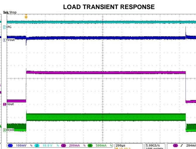
Figure 36. Power Save Mode, V_{IN}=12V , V_{OUT}=3.3V , I_{out} (50mA to 500mA)
