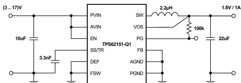
Figure 44. 1.8-V, 1-A Power Supply
