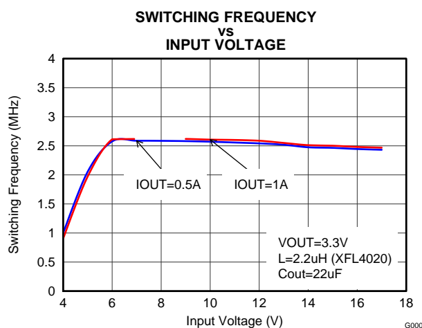
Figure 19. Switching Frequency
