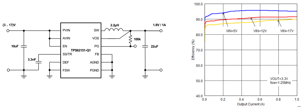
Figure 1. Typical Application and Efficiency
