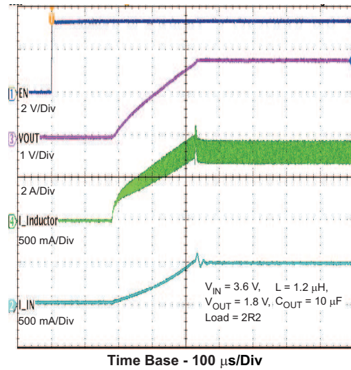
Figure 20. Startup Into Load – V_{OUT} 1.8 \text{ V}
