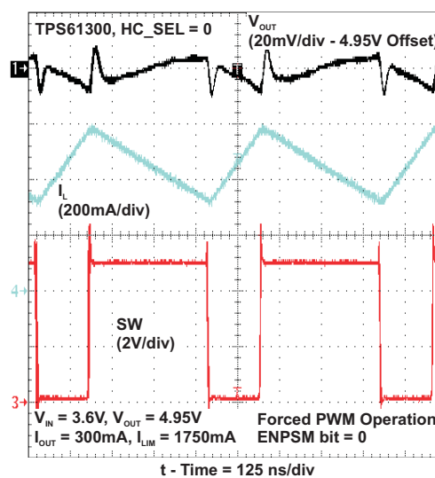
Figure 39. PWM OPERATION
