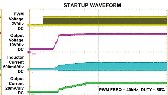
t - Time - 10ms/div Figure 8.
