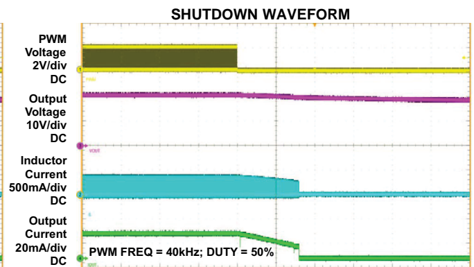
t - Time - 10ms/div Figure 10.
