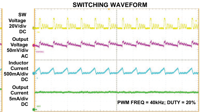
t - Time - 1 \mu s/div Figure 6.
