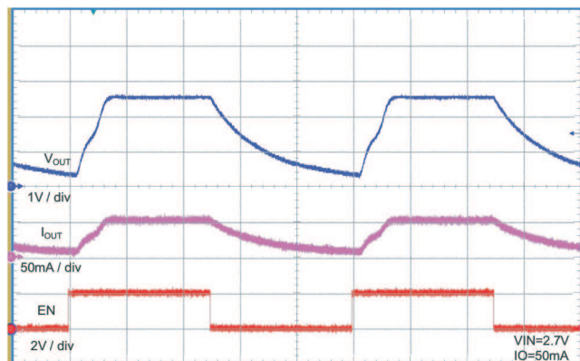
ENABLE / DISABLE V_{IN} = 2.7\text{ V} , I_O = 50\text{ mA}
