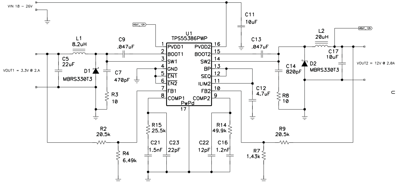
Figure 36. Design Example 2, TPS55386 in a Cascaded Configuration
