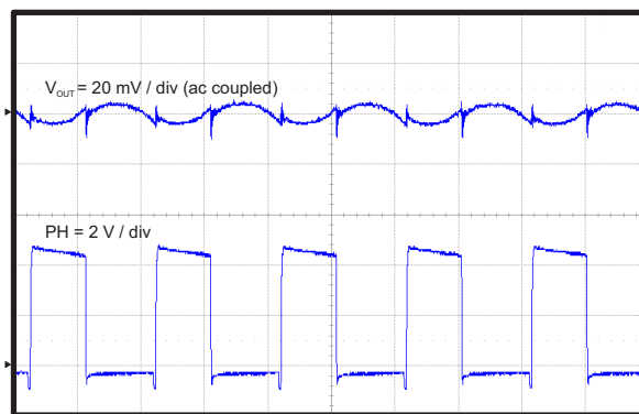
OUTPUT RIPPLE, I_{OUT} = 7 A
