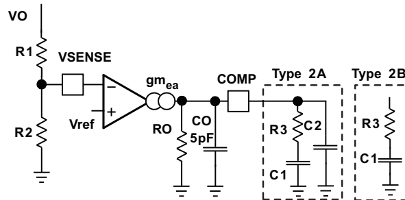
Figure 32. Types of Frequency Compensation
