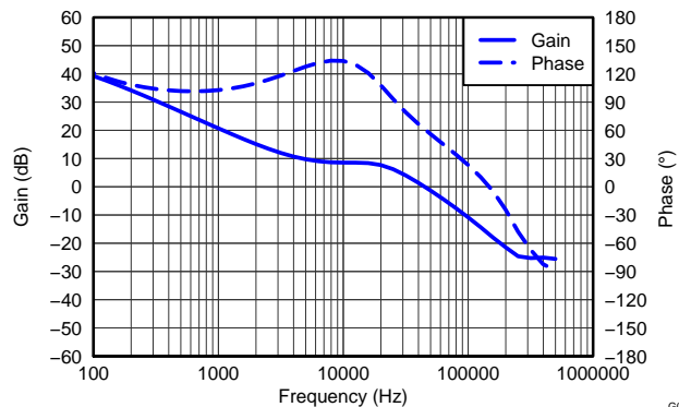
CLOSED LOOP RESPONSE, V_{IN} = 5 V, I_{OUT} = 3.5 A
