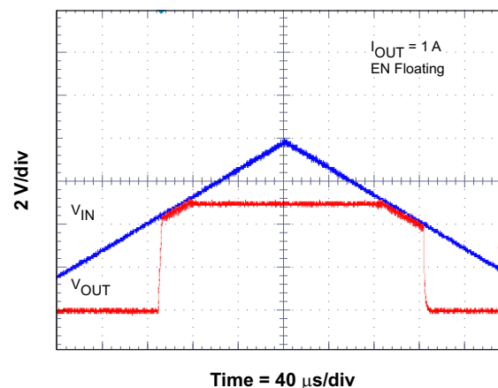
Figure 47. Low Dropout Operation
