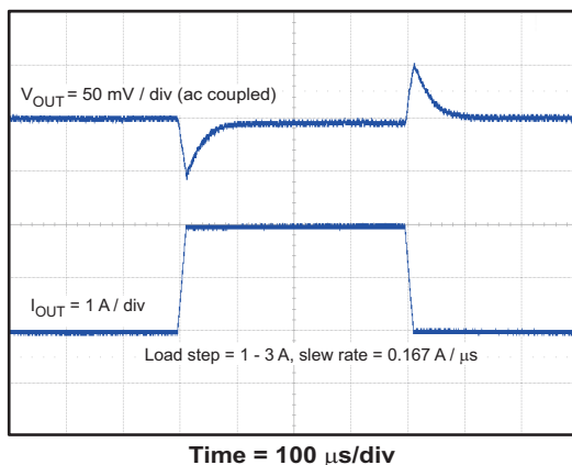
Figure 39. TRANSIENT RESPONSE, 2 A STEP
