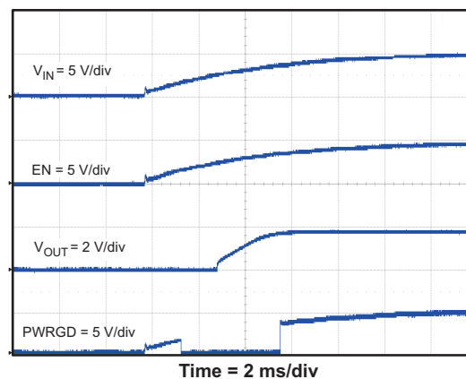
Figure 40. POWER UP VOUT, VIN
