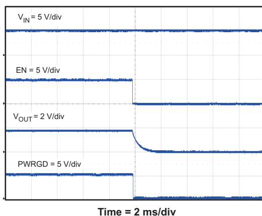
Figure 41. POWER UP VOUT, EN
