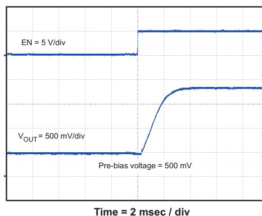
Figure 42. POWER UP INTO PRE-BIAS VOLTAGE
