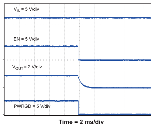
Figure 44. PWER DOWN VOUT, EN
