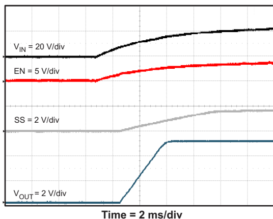
Figure 51. TPS54336 Start Up Relative to VIN
