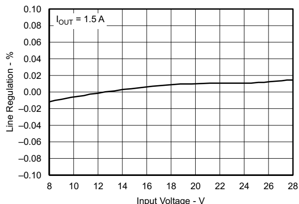
Figure 44. TPS54336 DRC Line Regulation
