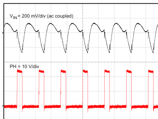
Figure 50. TPS54336 Full Load Input Ripple
