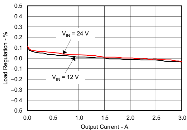
Figure 42. TPS54336 DRC Load Regulation
