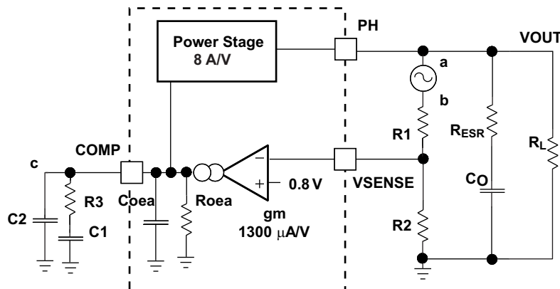
Figure 17. Small Signal Model for Loop Response
