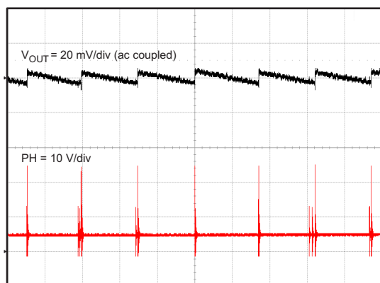
Figure 49. TPS54336 No Load Output Ripple
