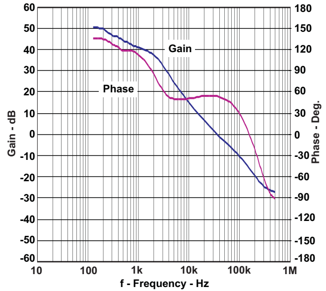
Figure 19. TPS54232 Loop Response
