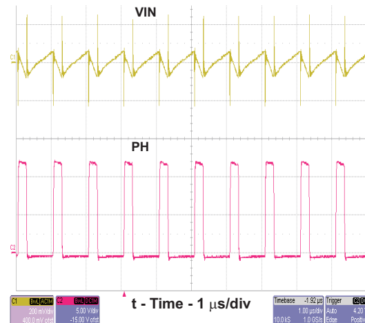
Figure 21. TPS54232 Input Ripple
