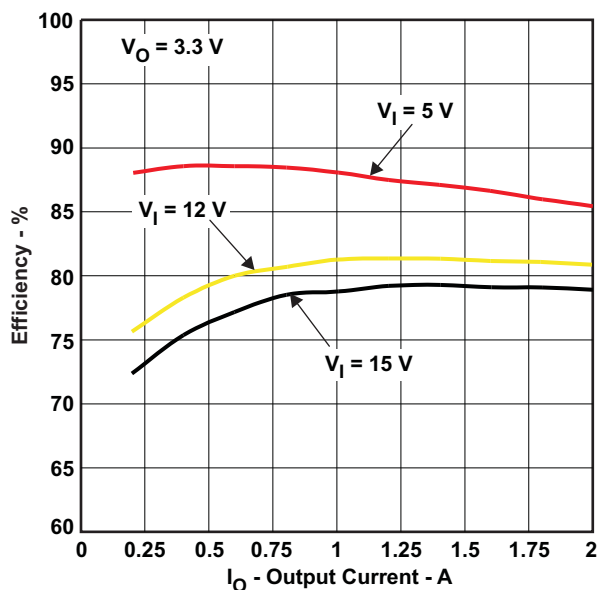
Figure 14. TPS54232 Efficiency
