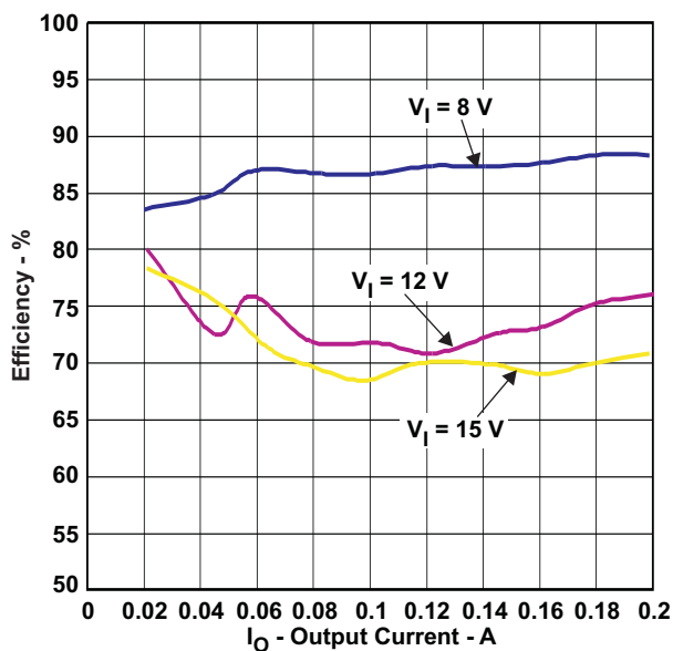
Figure 15. TPS54232 Low Current Efficiency
