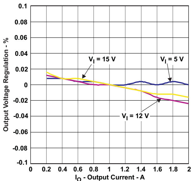
Figure 16. TPS54232 Load Regulation
