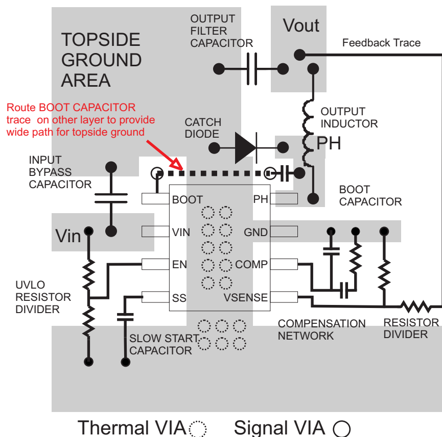
Figure 13. TPS54232 Board Layout
