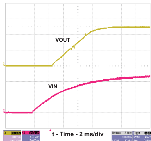
Figure 22. TPS54232 Start Up
