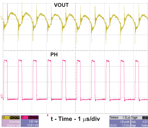
Figure 20. TPS54232 Output Ripple
