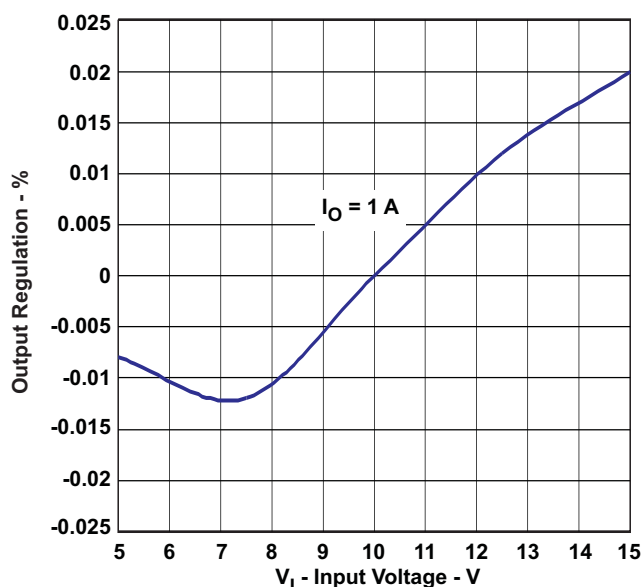
Figure 17. TPS54232 Line Regulation
