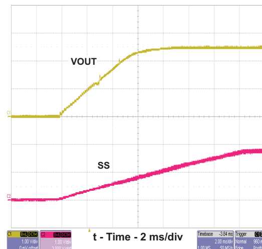
Figure 23. TPS54232 Start-up Relative to Enable
