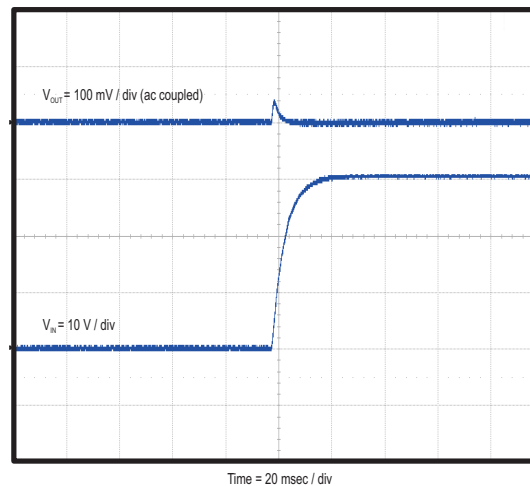
Figure 27. Line Transient
