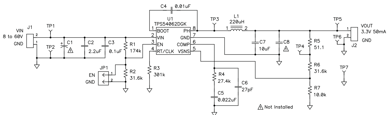
Figure 20. Application Schematic
