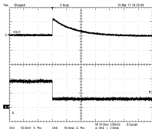
Figure 43. Unload Transient
