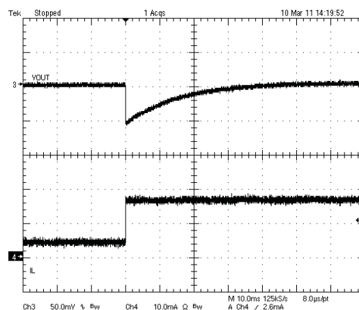
Figure 42. Load Transient
