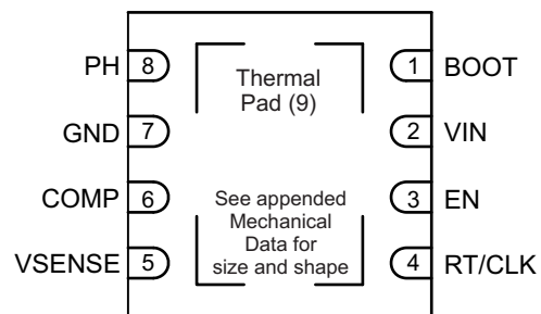
PIN CONFIGURATION VSON-8 PACKAGE (BOTTOM VIEW)
