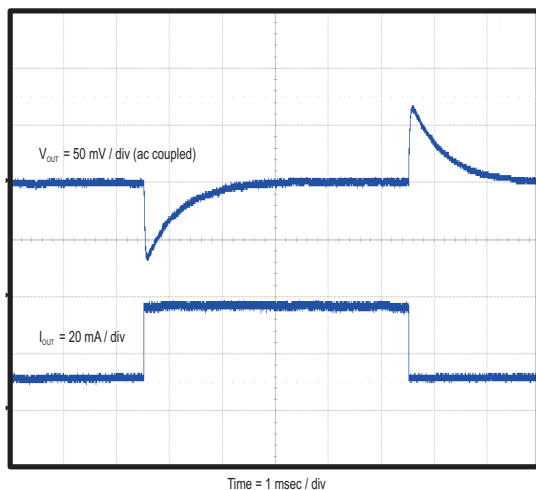
Figure 26. Load Transient
