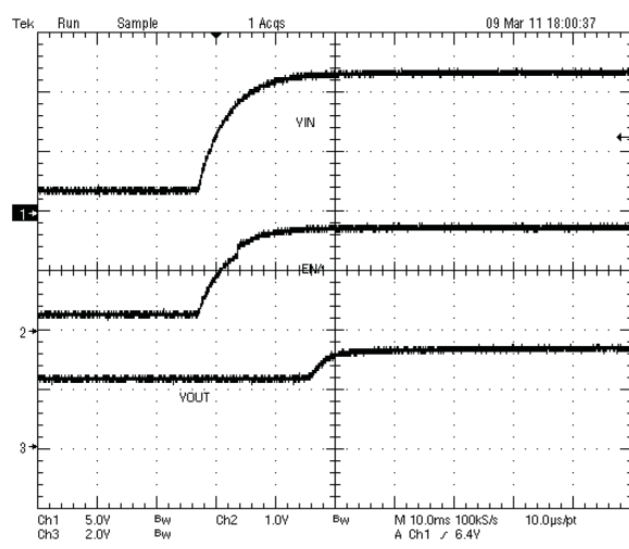
Figure 47. Prebias Startup With V_{IN}
