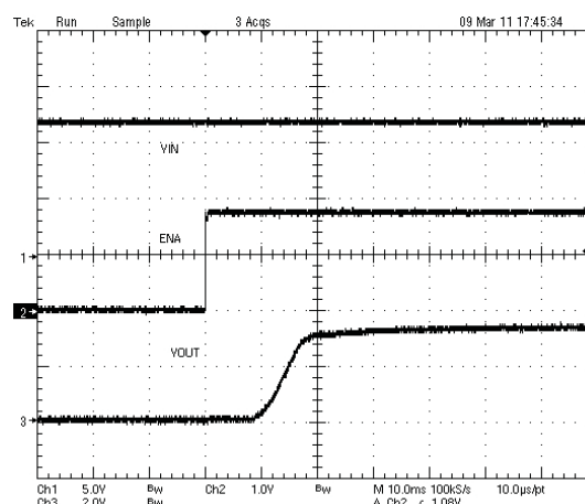
Figure 44. Startup With ENA
