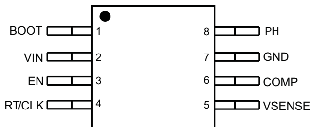
PIN CONFIGURATION MSOP-8 PACKAGE (TOP VIEW)
