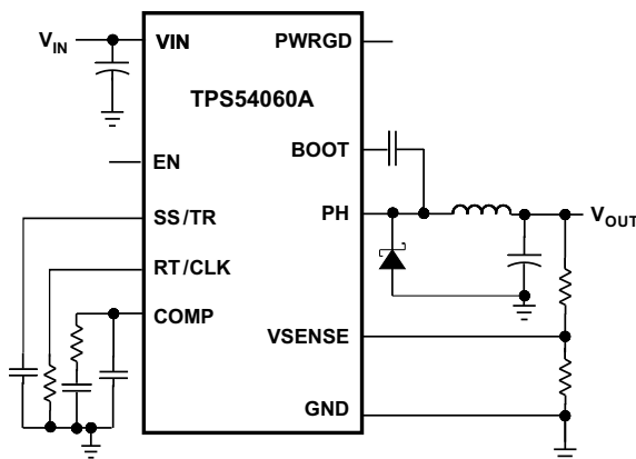
SIMPLIFIED SCHEMATIC
