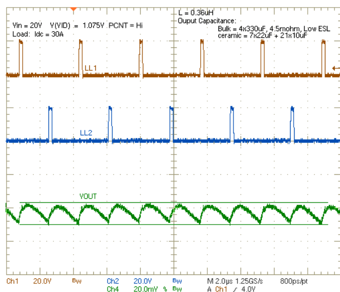
Figure 30. Output Ripple, V_{IN} = 20\text{ V}
