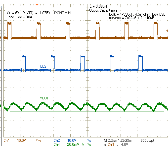
Figure 31. Output Ripple, V_{IN} = 9\text{ V}
