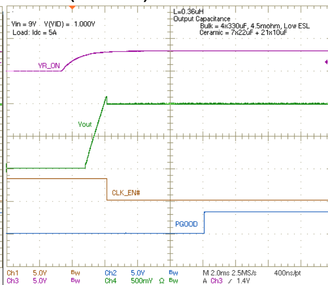
Figure 29. \overline{PG} and PGOOD , V_{IN} = 9\text{ V}
