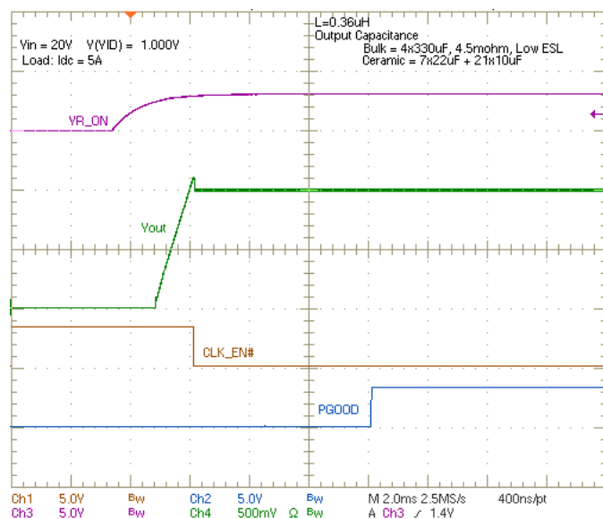
Figure 28. \overline{PG} and PGOOD , V_{IN} = 20\text{ V}
