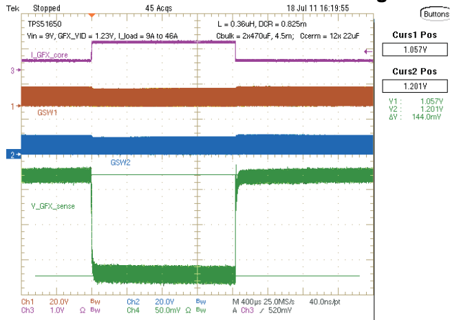
Figure 25. Load Transient, V IN = 9 V, Load Step = 37 A
