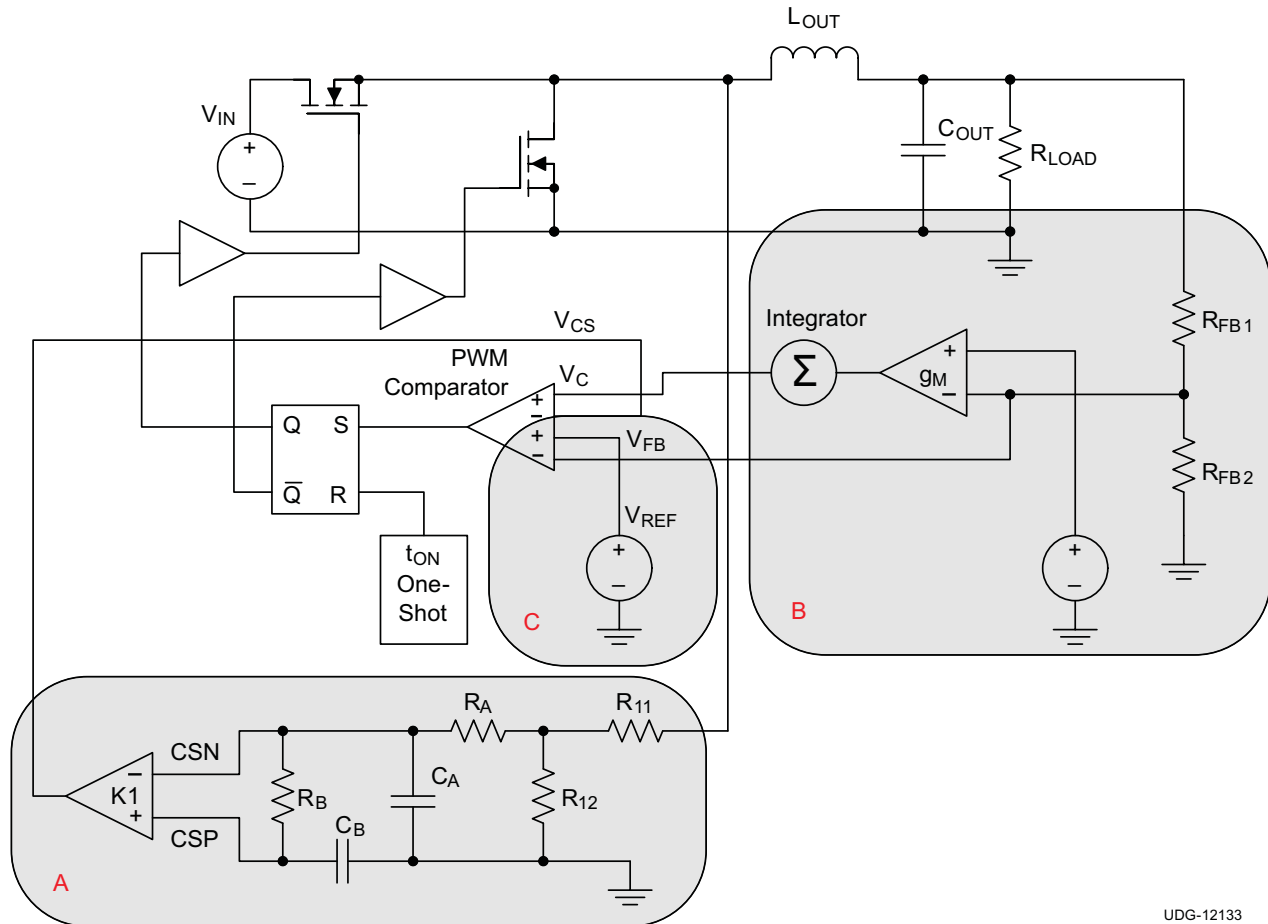
Figure 9. 3/4 PWM Operation
