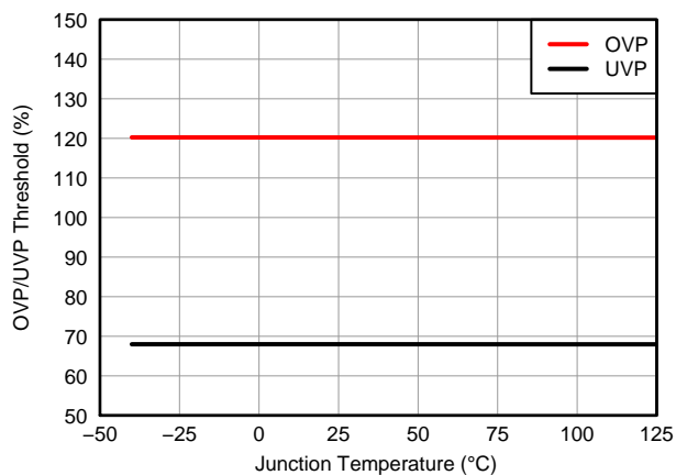
Figure 5. OVP/UVLP Threshold vs Junction Temperature
