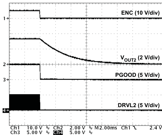
3.3-V Soft-stop Waveforms
