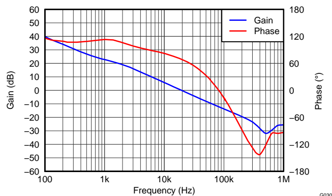
Figure 31. Loop Gain and Phase
