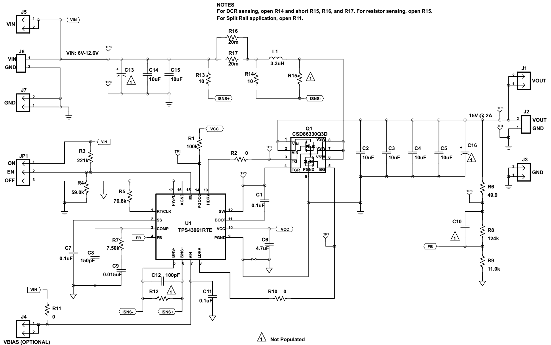
Figure 21. The Schematic of Synchronous Boost Converter using TPS43061
