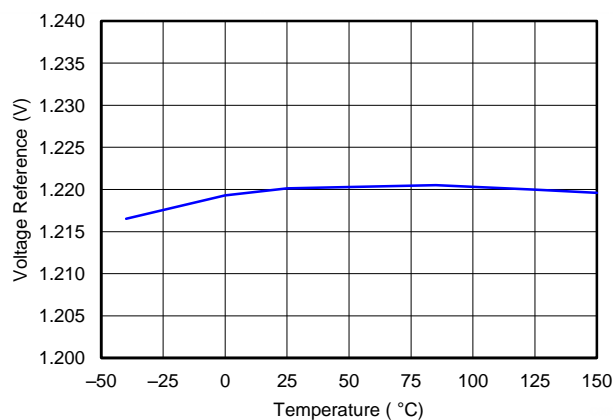
Figure 5. Feedback Voltage Reference vs Temperature
