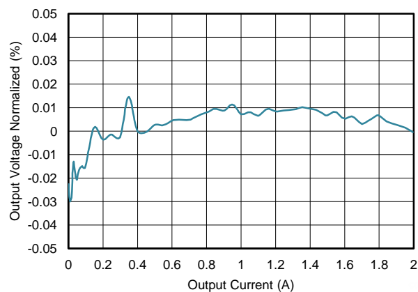
Figure 32. Load Regulation
