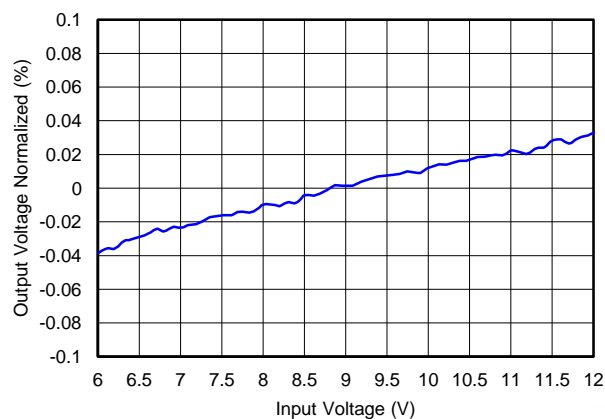
Figure 33. Line Regulation
