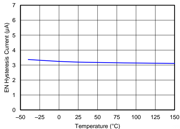
Figure 8. EN Hysteresis Current vs Temperature
