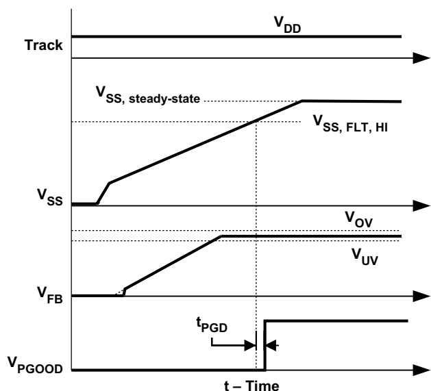
Figure 34. PGOOD Signal
