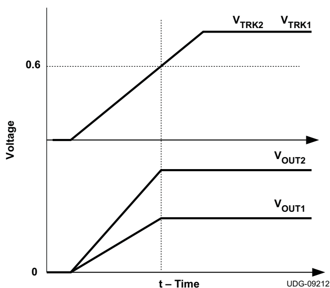
Figure 30. Ratiometric Voltage Tracking Waveform
